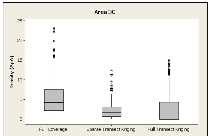
Figure 15. Box and whisker plots for full-coverage areas 3A, 3B, and 3C, comparing anomaly density values from the ground-based magnetometry survey, and the sparse and full transect kriging estimates. Figure on left shows the locations of the full-coverage areas highlighted with red rectangle.
