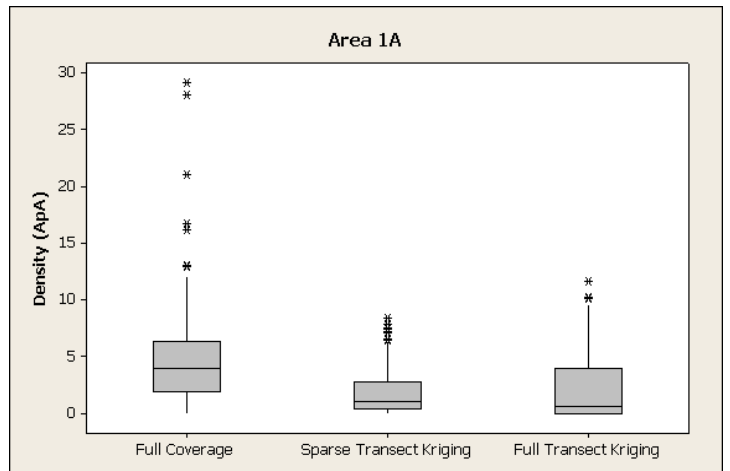
Figure 13. Box and whisker plots for full-coverage areas 1A, 1B, and 1C, comparing anomaly density values from the ground-based magnetometry survey, and the sparse and full transect kriging estimates. Figure on left shows the locations of the full-coverage areas highlighted with red rectangle.
