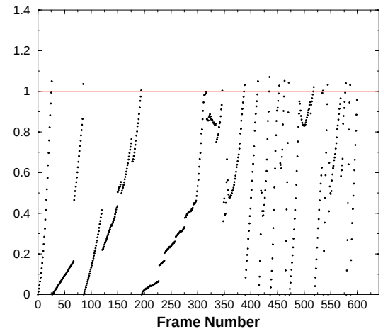
Error (pixels)
