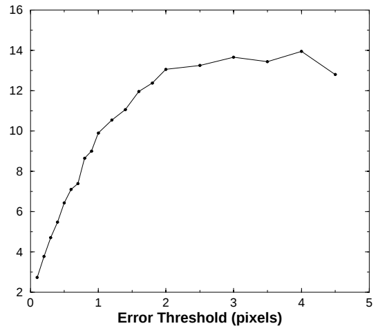
Speedup
