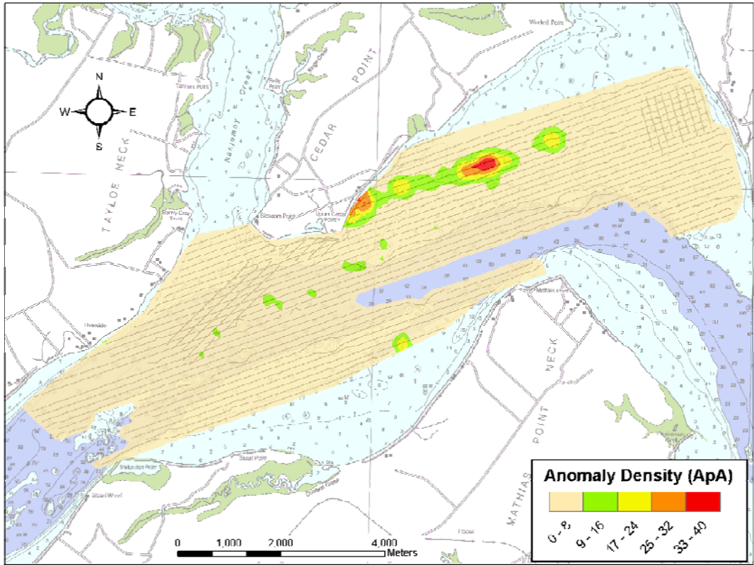
Figure 12. Anomaly density values (ApA) for the Blossom Point study area. Areas without anomaly density color shading were not estimated because observational data were not available.
