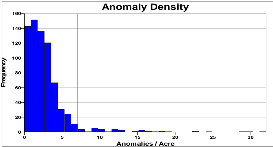
Figure A-1. Flagged high-density regions from a 500-m diameter window using a 7-ApA critical density (top) and the histogram of site densities with a red line marking 7 ApA (bottom).
