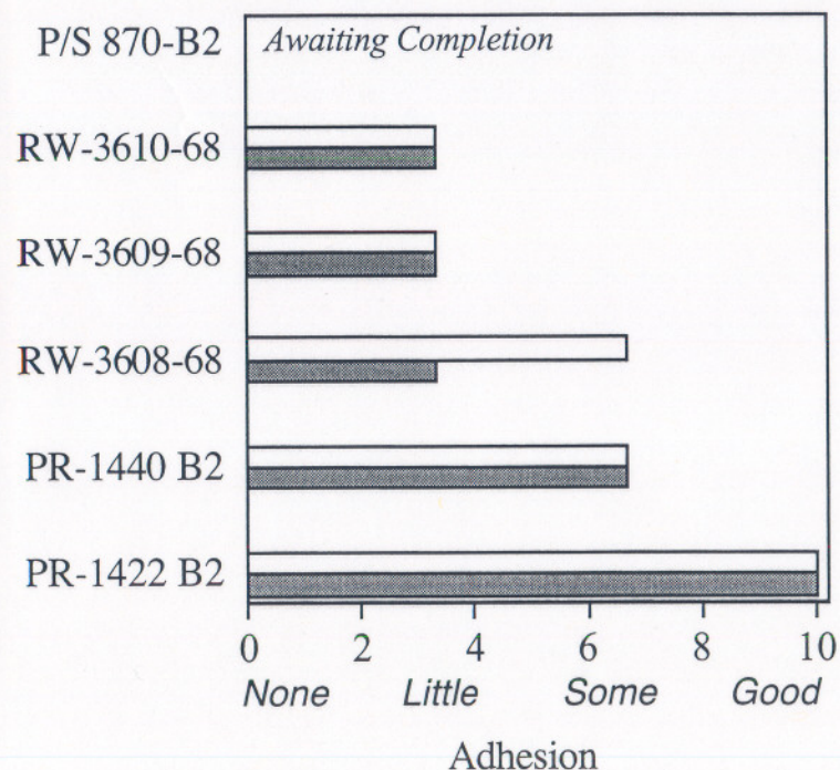
3 mm Scribe Adhesion @3 Weeks ASTM B 117
