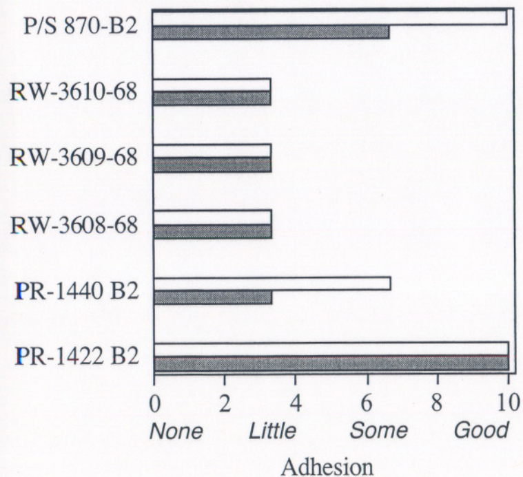
3 mm Scribe Adhesion @1 Week ASTM G 85
