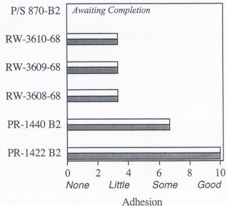
5 mm Scribe Adhesion @3 Weeks ASTM B 117
