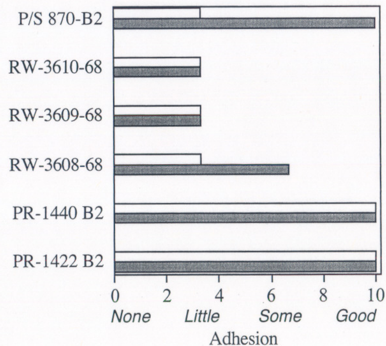
5 mm Scribe Adhesion @1 Week ASTM G 85
