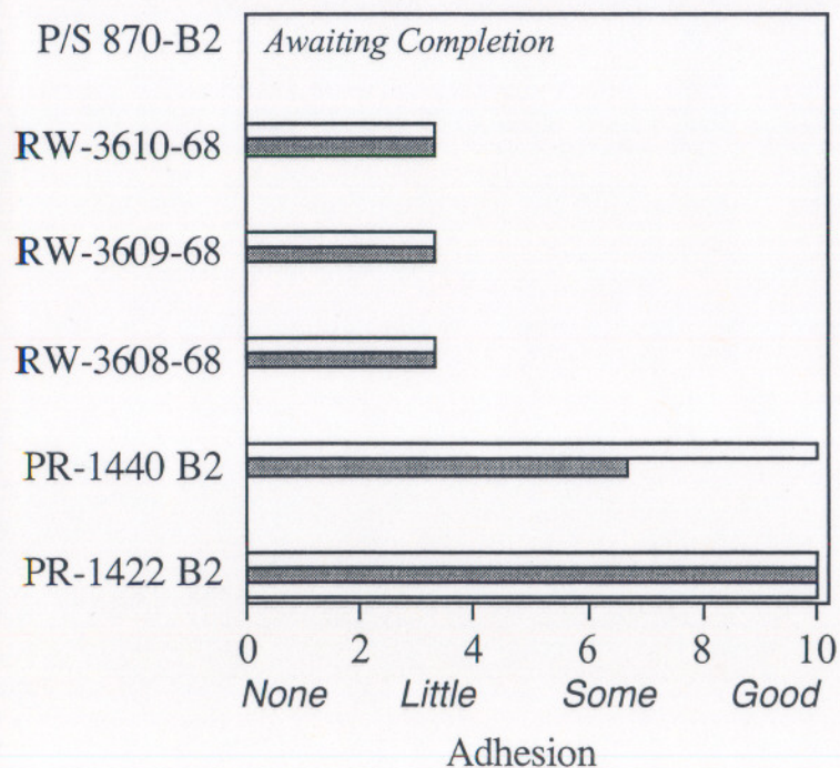
3 mm Scribe Adhesion @2 Weeks ASTM G 85
