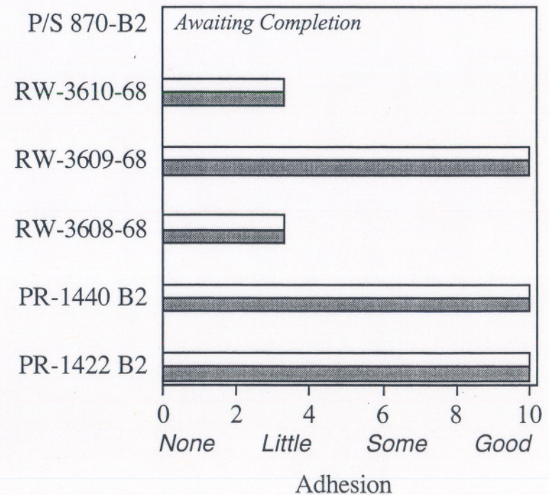
5 mm Scribe Adhesion @4 Weeks ASTM B 117
