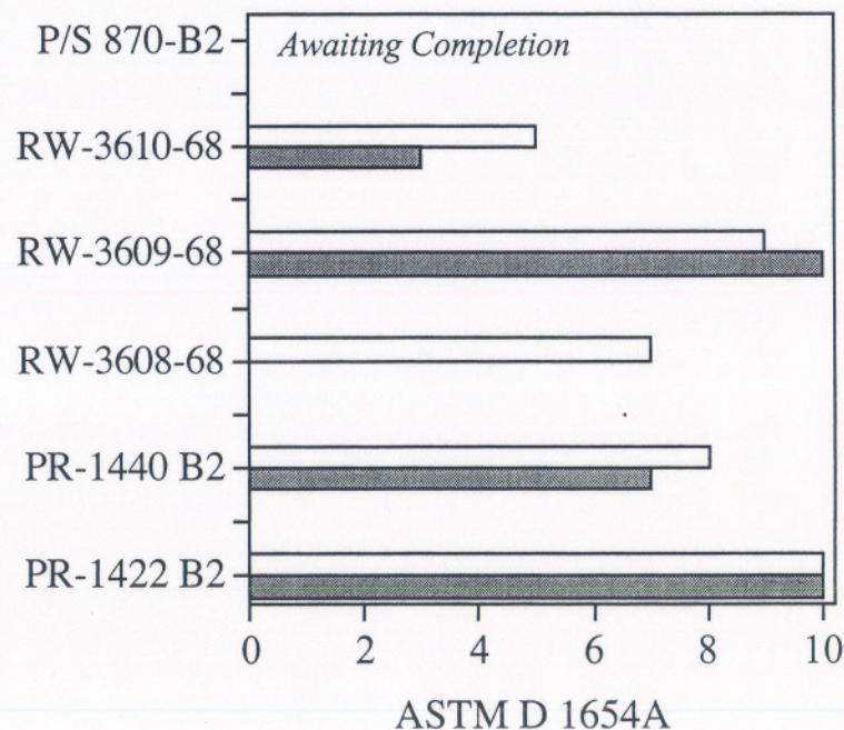
Corrosion Ingress from 5 mm Scribe @3 Weeks ASTM G 85
