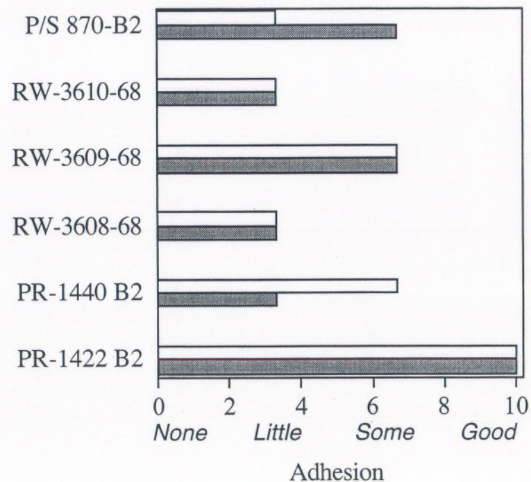
5 mm Scribe Adhesion @1 Week ASTM B 117
