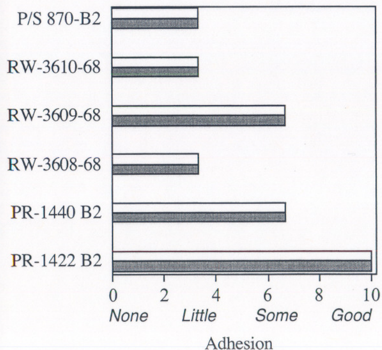
3 mm Scribe Adhesion @2 Weeks ASTM B 117
