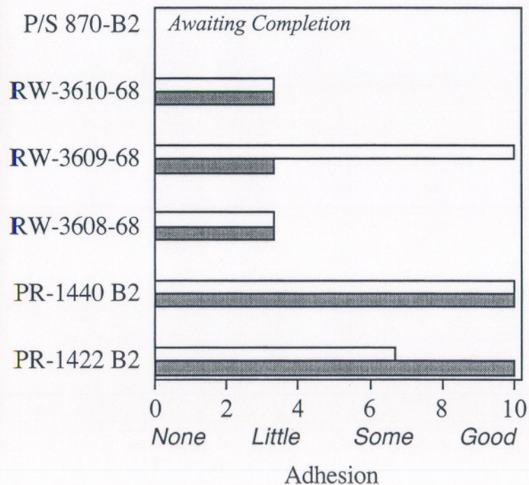
3 mm Scribe Adhesion @4 Weeks ASTM B 117
