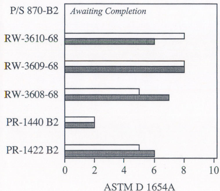
Corrosion Ingress from 3 mm Scribe @6 Weeks ASTM G 85
