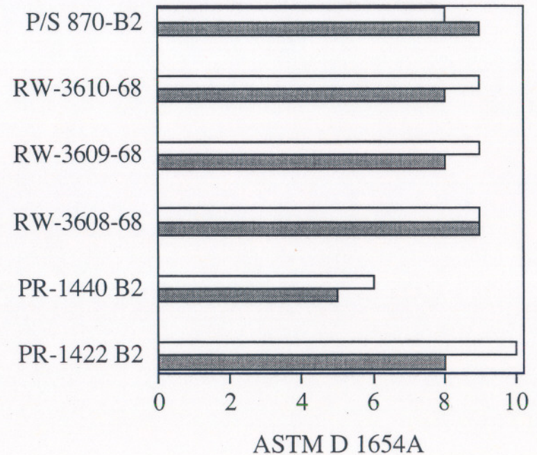
Corrosion Ingress from 5 mm Scribe @2 Weeks ASTM B 117
