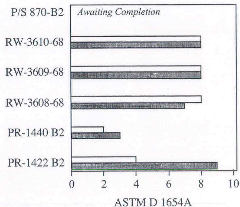
Corrosion Ingress from 5 mm Scribe @5 Weeks ASTM B 117
