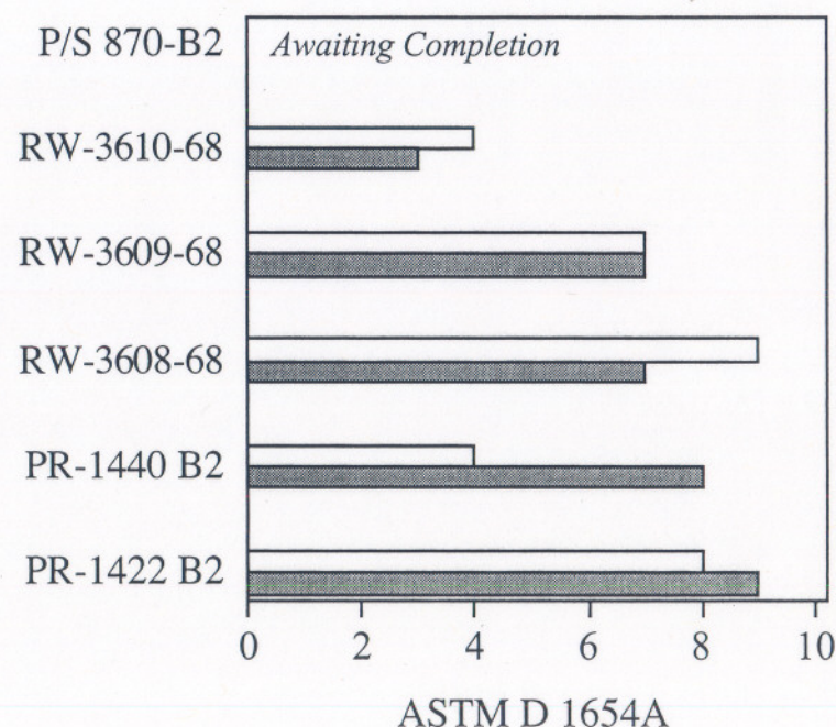
Corrosion Ingress from 5 mm Scribe @5 Weeks ASTM G 85
