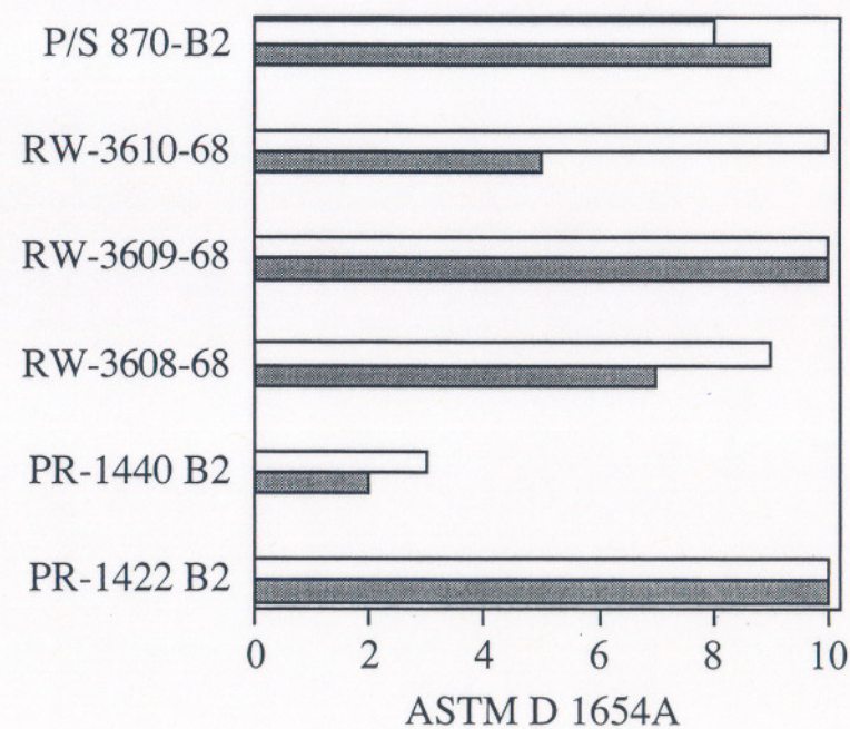
Corrosion Ingress from 5 mm Scribe @1 Week ASTM B 117
