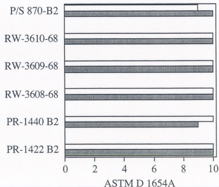
Corrosion Ingress from 5 mm Scribe @1 Week ASTM G 85
