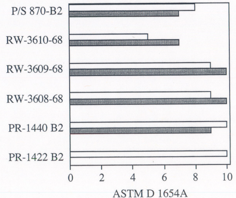
Corrosion Ingress from 5 mm Scribe @2 Weeks ASTM G 85
