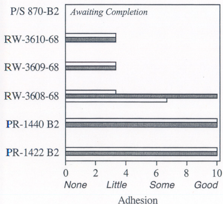
3 mm Scribe Adhesion @3 Weeks ASTM G 85
