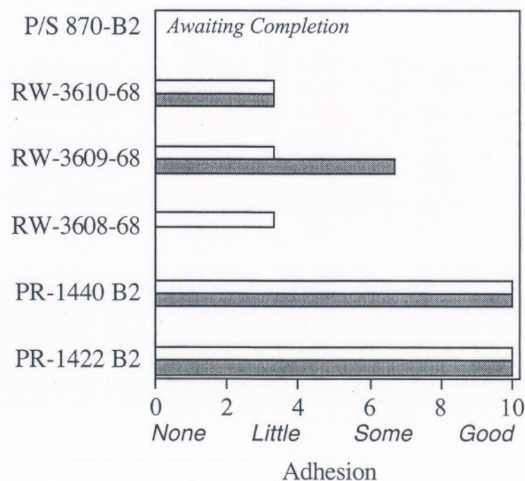
5 mm Scribe Adhesion @3 Weeks ASTM G 85
