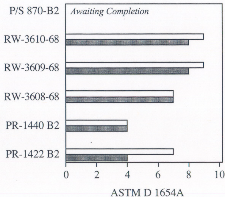
Corrosion Ingress from 5 mm Scribe @6 Weeks ASTM B 117
