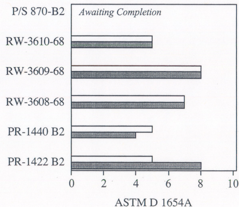
Corrosion Ingress from 5 mm Scribe @6 Weeks ASTM G 85
