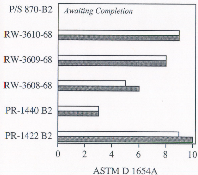
Corrosion Ingress from 3 mm Scribe @4 Weeks ASTM B 117
