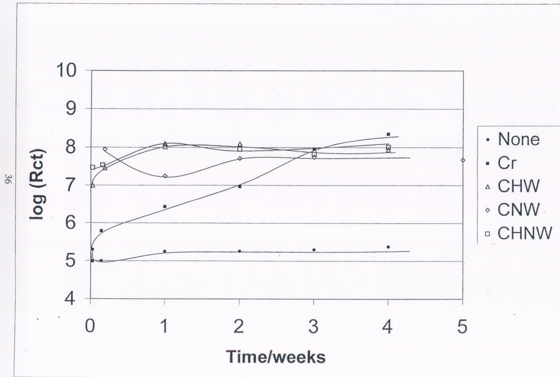
Figure 15: EIS Curves of Sealants with CHW, CNW, and CHNW on 2024
