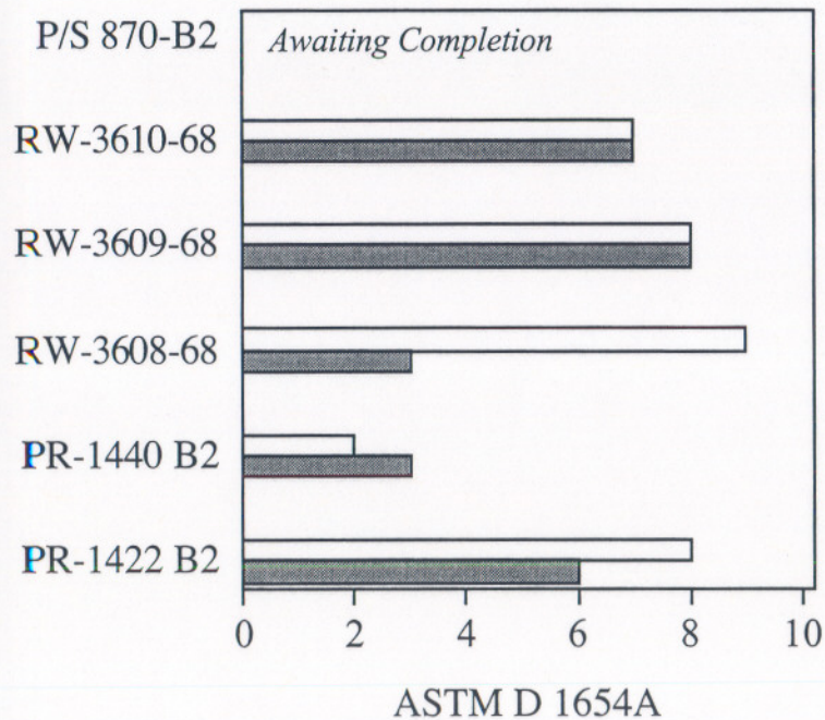
Corrosion Ingress from 3 mm Scribe @3 Weeks ASTM B 117
