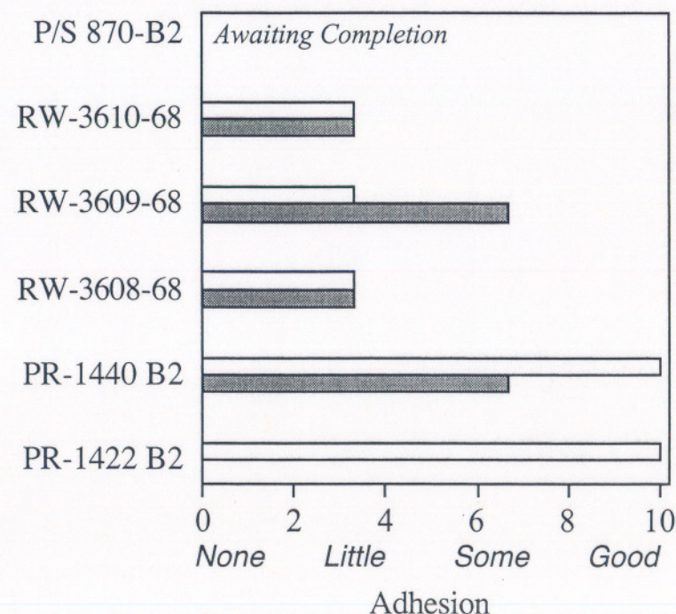
5 mm Scribe Adhesion @2 Weeks ASTM G 85
