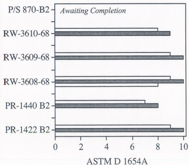
Corrosion Ingress from 3 mm Scribe @3 Weeks ASTM G 85
