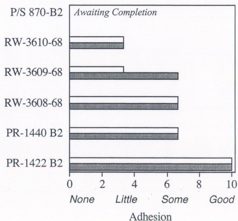
5 mm Scribe Adhesion @6 Weeks ASTM B 117
