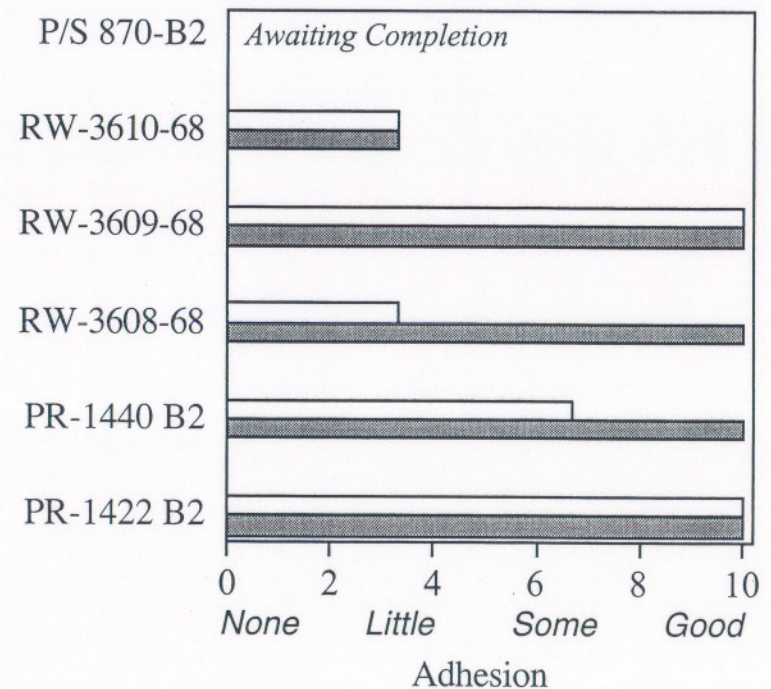
5 mm Scribe Adhesion @6 Weeks ASTM G 85
