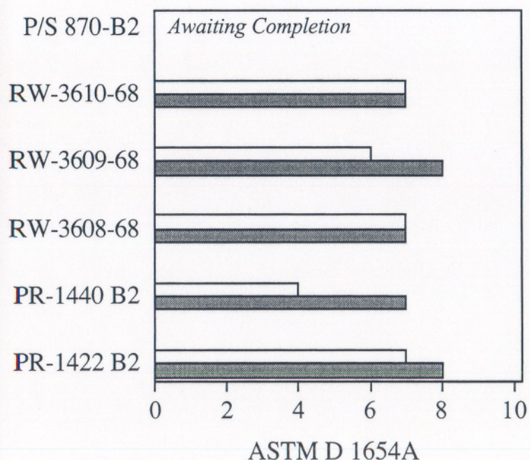
Corrosion Ingress from 3 mm Scribe @5 Weeks ASTM G 85
