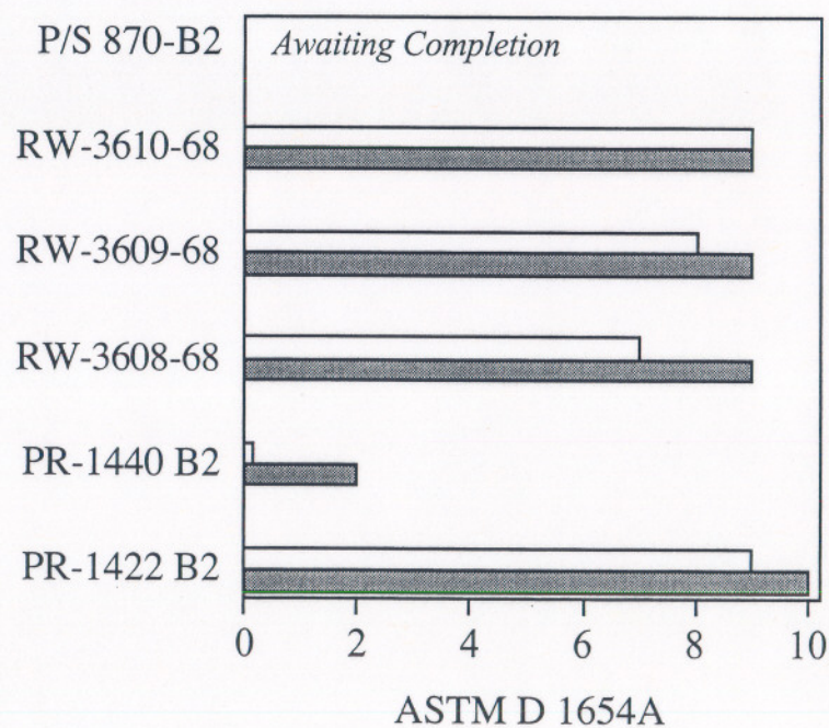
Corrosion Ingress from 5 mm Scribe @4 Weeks ASTM B 117
