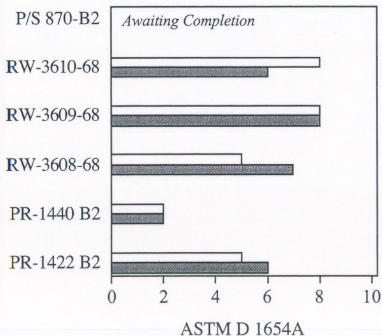
Corrosion Ingress from 3 mm Scribe @6 Weeks ASTM B 117
