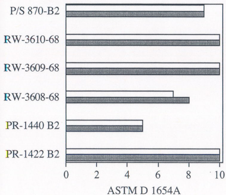
Corrosion Ingress from 3 mm Scribe @1 Week ASTM B 117
