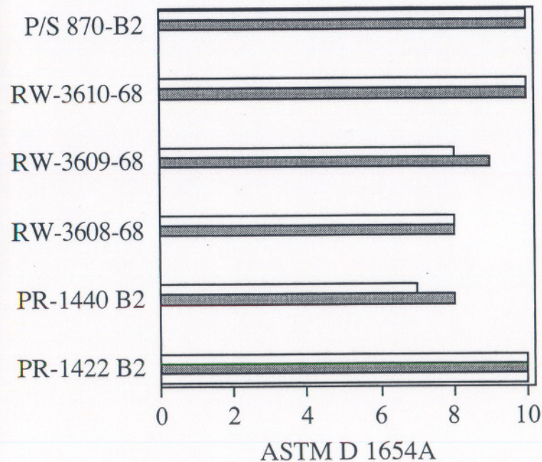
Corrosion Ingress from 3 mm Scribe @2 Weeks ASTM G 85
