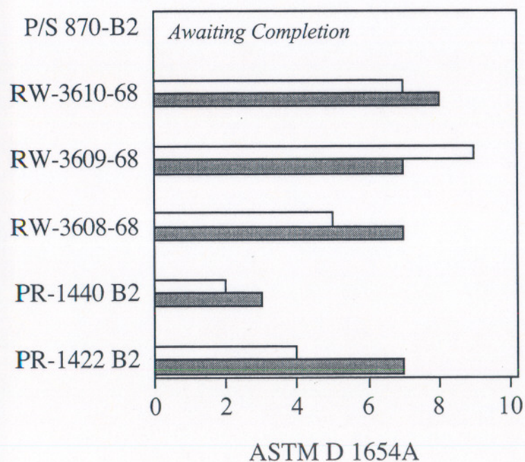
Corrosion Ingress from 3 mm Scribe @5 Weeks ASTM B 117
