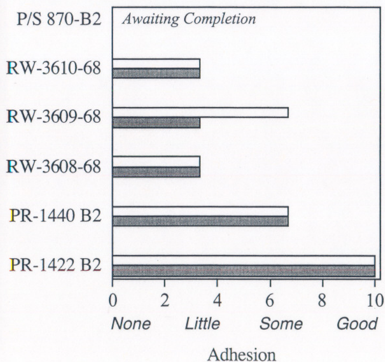
3 mm Scribe Adhesion @6 Weeks ASTM B 117
