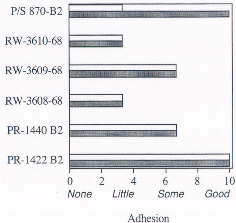
5 mm Scribe Adhesion @2 Weeks ASTM B 117
