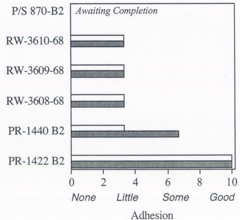
5 mm Scribe Adhesion @5 Weeks ASTM B 117
