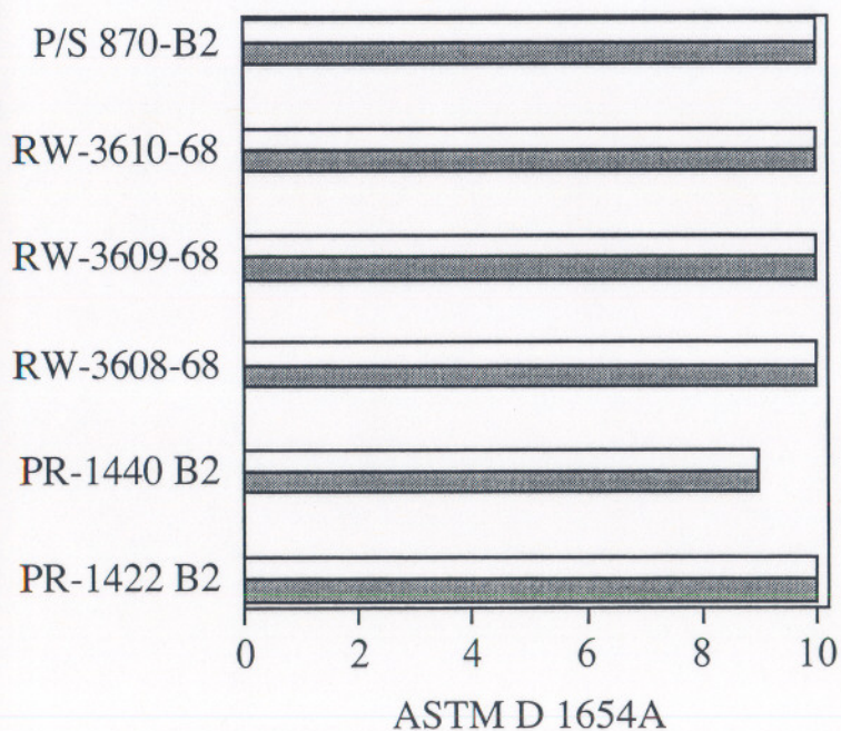
Corrosion Ingress from 3 mm Scribe @1 Week ASTM G 85
