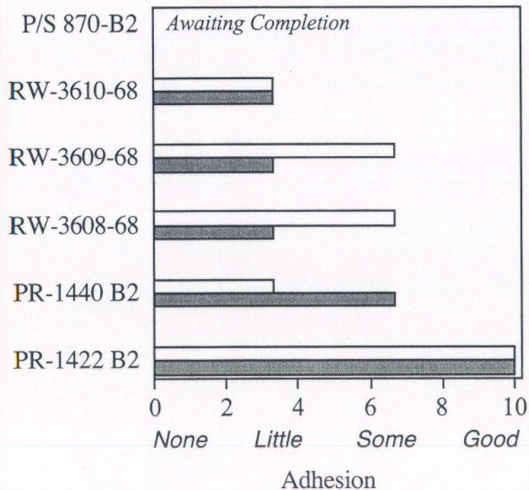
3 mm Scribe Adhesion @5 Weeks ASTM B 117
