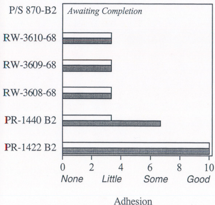
3 mm Scribe Adhesion @5 Weeks ASTM G 85
