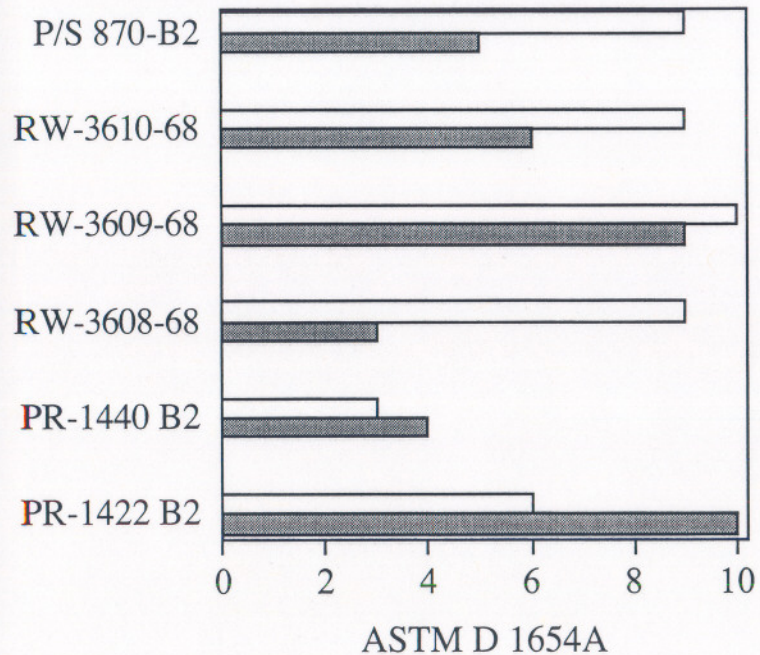
Corrosion Ingress from 3 mm Scribe @2 Weeks ASTM B 117
