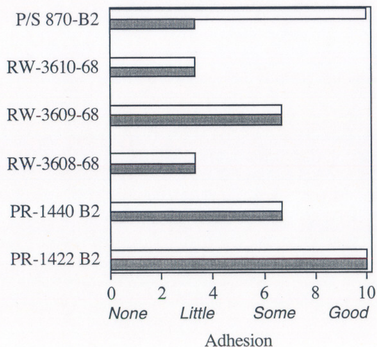
3 mm Scribe Adhesion @1 Week ASTM B 117
