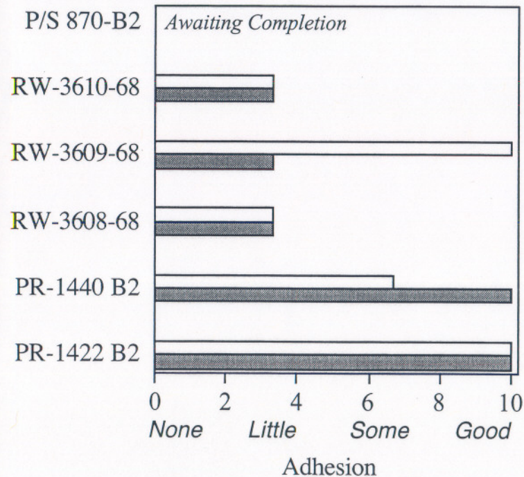
3 mm Scribe Adhesion @6 Weeks ASTM G 85
