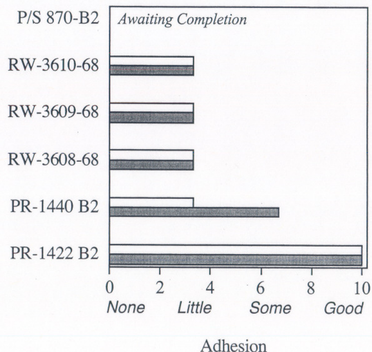
5 mm Scribe Adhesion @5 Weeks ASTM G 85
