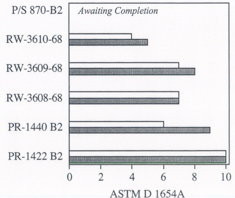
Corrosion Ingress from 5 mm Scribe @4 Weeks ASTM G 85
