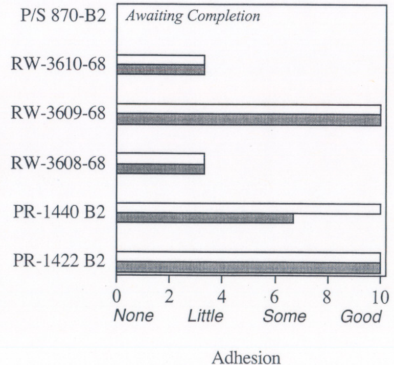
5 mm Scribe Adhesion @4 Weeks ASTM G 85
