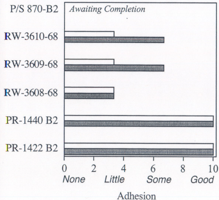
3 mm Scribe Adhesion @4 Weeks ASTM G 85
