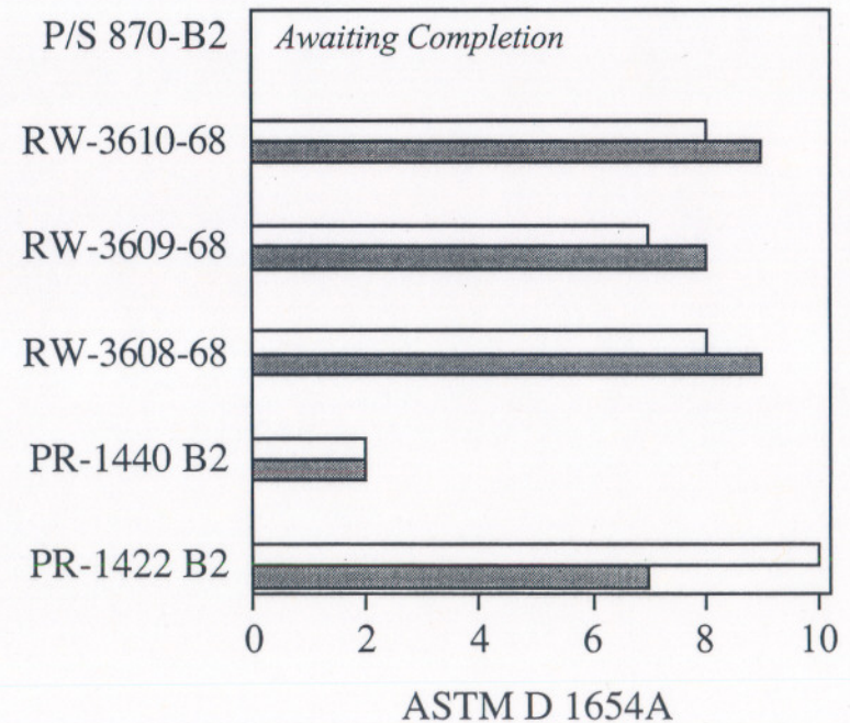
Corrosion Ingress from 5 mm Scribe @3 Weeks ASTM B 117
