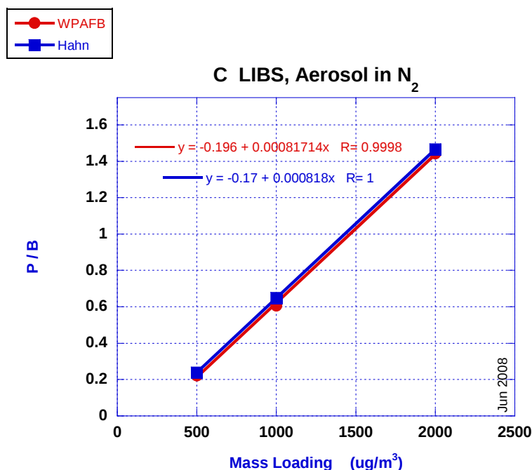
Figure 4.2.10. Comparison of peak-to-base ratios for carbon in aerosol form (oxalic acid) versus mass loading for the data collected with the setup at WPAFB and at the Univ. of Florida (Hahn). Backward light collection.
