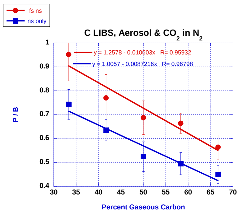
Figure 4.2.17. Peak-to-base ratios for fs-ns and ns-only excitation of carbon in CO 2 /aerosol mixtures as a function of the percent of gaseous carbon present. Downward slopes are indicative of stronger LIBS signals from the aerosol phase. For each mixture, the total mass loading of all carbon present was held to 5000 µg/m 3 .
