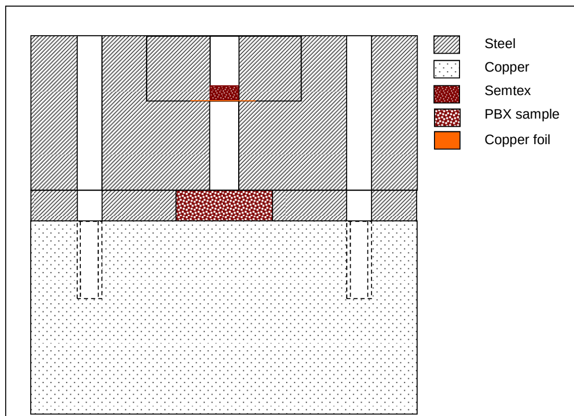
Schematics of the (modified) Floret test as used at TNO.
