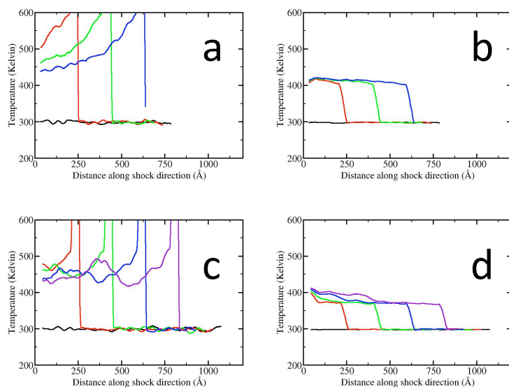
FIG. 4. Instantaneous spatial profiles for intermolecular (panels (a) and (c)) and intramolecular (panels (b) and (d)) temperature at 5.0 ps intervals starting from the time of shock initiation in the flexible slabs ( t = 0 ). Panels (a) and (b): [001] shock; panels (c) and (d): [100] shock.
