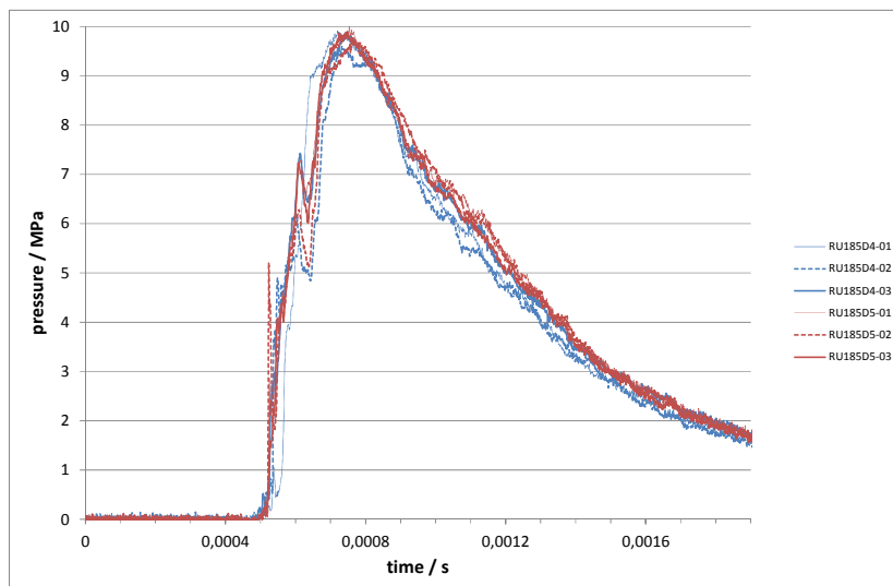
Mechanical response of 3.5 mm Ø X 2.5 mm RU185 samples (containing RDX-K7) in BIC tests in triplicate experiments. Samples were taken from the explosion driven deformation tests with a 4 mm (RU185D4-xx) or 5 mm (RU185D5-xx) plastic explosive layer. Time scales are relative to the start of deformation measured for each individual experiment.
