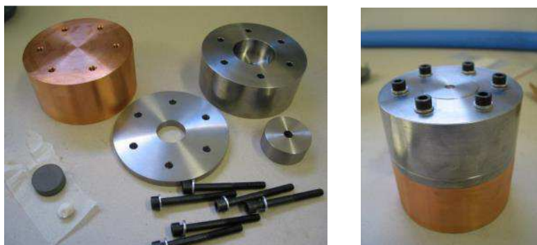
Pictures of disassembled (left) and assembled (right) Floret test set-up. The left picture also shows a PBX sample.
