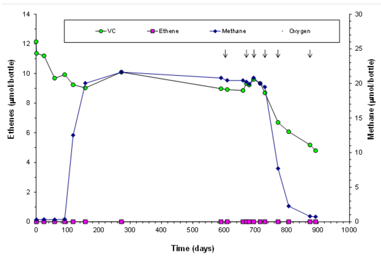
Figure 5.5. Results for a Site #2, Set I-A microcosm that was switched from anaerobic to aerobic conditions on day 604 by adding oxygen; each arrow represent 0.1 mL of oxygen (ca. 4 μmol).
