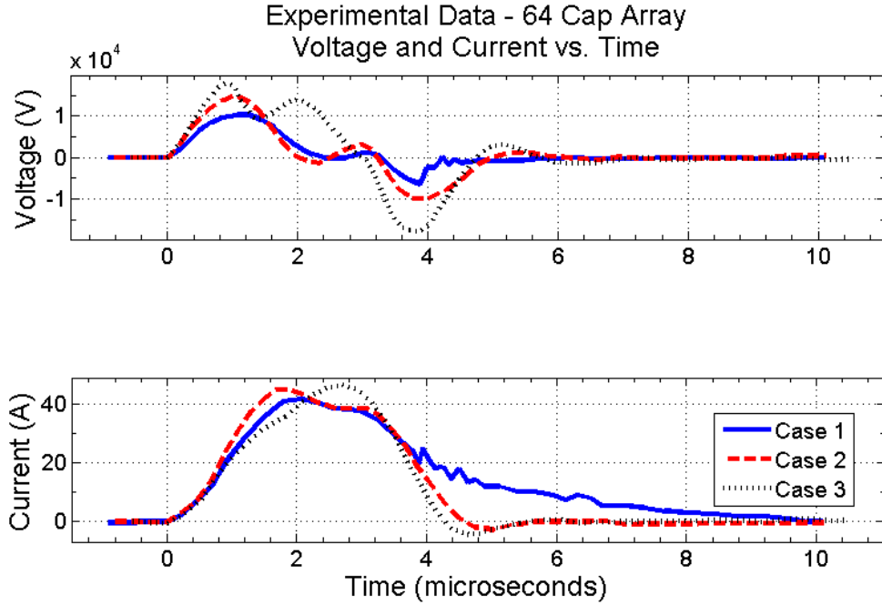
Figure 16. Experimental data showing all three 64-blasting cap tests with coincident time axis.
