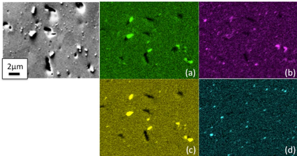
Figure 47. EDX map for welding condition 400RPM/50MMPPM showing the concentration of (a) oxygen, (b) yttrium, (c) aluminum and (d) titanium.
