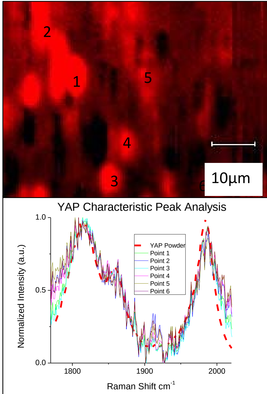
Figure 33. YAP found in 500RPM/25MMPPM FSW condition at multiple points in the measured area versus YAP powder.
