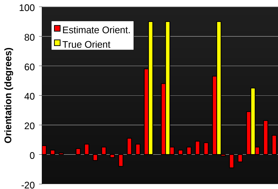
Figure 39. Comparison of estimated orientation and true orientation of correctly classified UXO-like items
