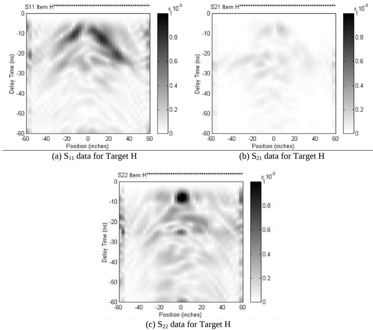
Figure 16 Preprocessed GPR data for Target H (horizontal plate, 4"x 4"x 0.25").
