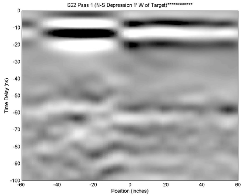
Figure 44c. S 22
