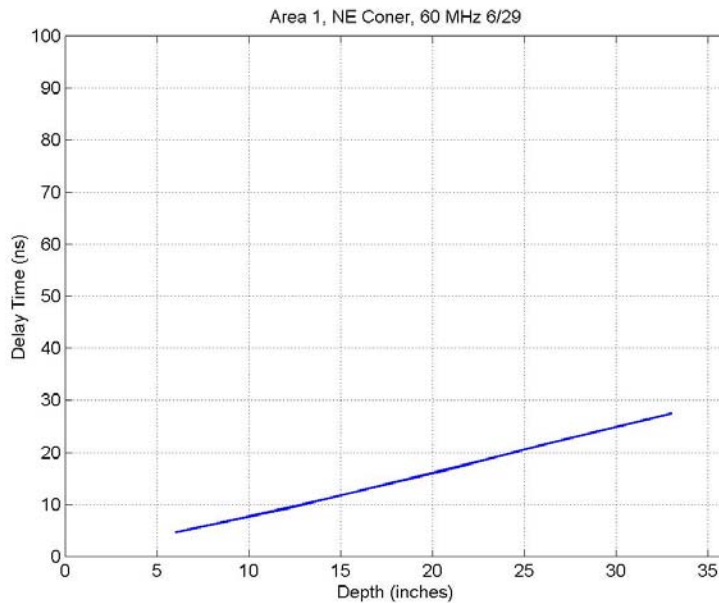
Figure 15 Predicted delay time as a function of depth in Area 1 of JPG V on 6/29/01.
