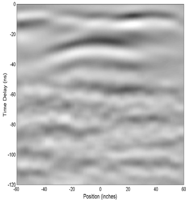
Figure 10 Measured Data for Known Target 2-126 with Antenna Calibration.
