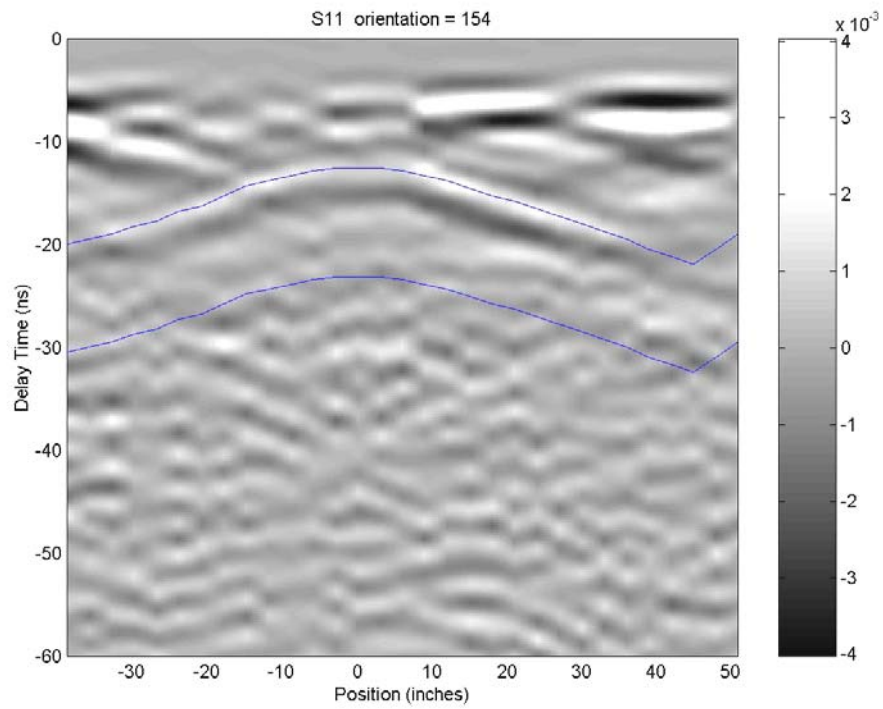
Figure 36a. Filtered S11 Responses
