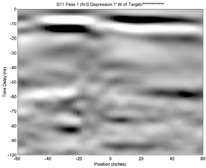
Figure 44a. S_{11}
