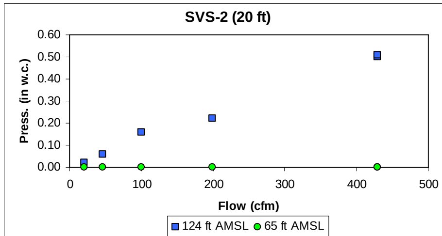
Figure 5-3 Effect of Air Flow on Pressure at Piezometer SVS-2.
