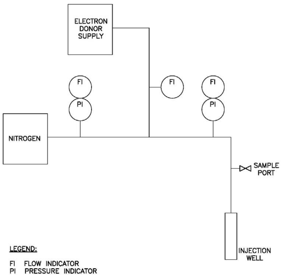
Figure 2 – Example Gas Injection GEDIT Process and Instrumentation Diagram
