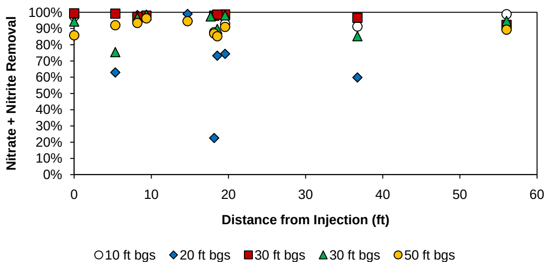
Figure 59 – Nitrate/Nitrite Removal Based on All Data
