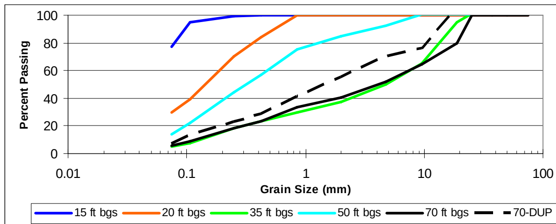
Figure 2-4 CDM-INJ1 Grain Size Distribution
