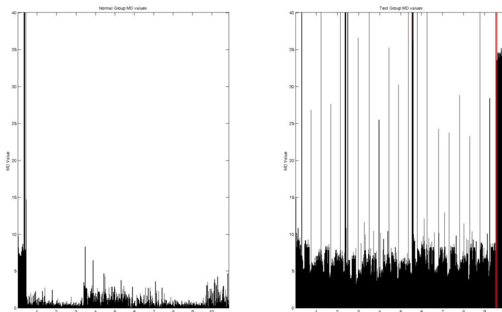
Figure 5: MD values from the normal (left) and abnormal (right) data with initial 4-factors
