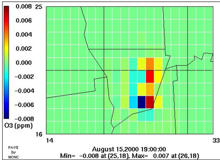
Figure 4 Static Grid Result for Brute Force Sensitivity of O 3 (ppm) to Fire Emissions
