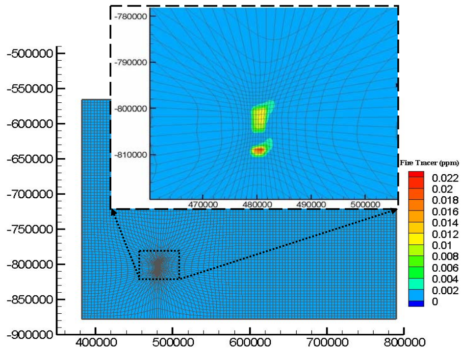
Figure 3 Adaptive Grid Result for Inert Fire Tracer Concentrations (ppm)
