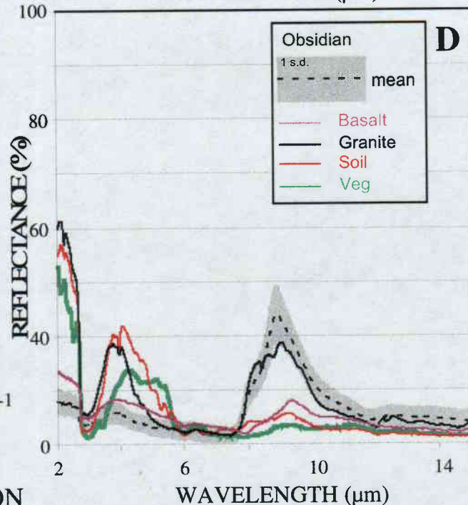
Figure 6: Detection thresholds for pottery sherds (A) and obsidian artifacts (B) using the full range of laboratory spectra (2 - 15 \mu m). The results for each substrate background (in mixtures with vegetation) are shown as: 1) soil (red), 2) granite (black), and 3) basalt (purple). The spectra used in the analysis are shown in C (pottery and backgrounds) and D (obsidian and backgrounds). The mean spectrum for the artifacts is shown as a black dashed line with the standard deviation in gray.
