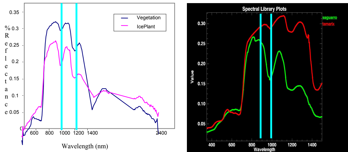
Figure 3: The bands used by the water band index (WBI) for sample vegetation at VAFB (left) and Yuma Proving Ground (right).
