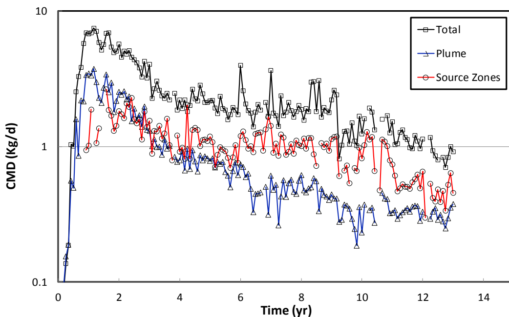
Figure 5.3.2-4. Contaminant mass discharge for the first 13 years as a function of source; time zero corresponds to the start of the pump-and-treat operation (April 1987).
