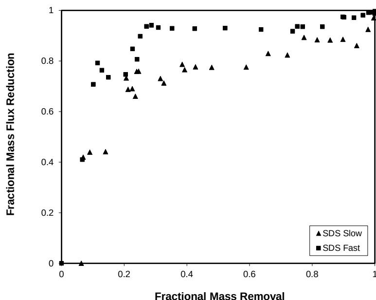
Figure 5.1.1-11. Relationship between reductions in mass flux and mass for data presented in Figure 5.1.1-10.
