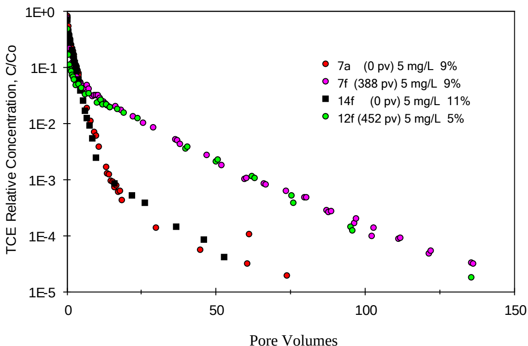
Figure 5.3.1-6. TCE Elution curves for systems flooded with potassium nitrate solution. There are two pairs of data. One set represent controls with no flooding prior to the experiments; these are denoted with (0) in the legend. The other set were flooded with ~400 pore volumes of potassium nitrate solution.
