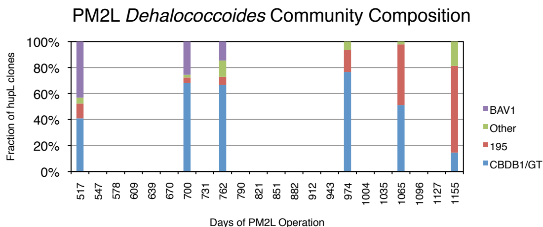
Figure 24 – Dehalococcoides community composition in the PM2L chemostat as assessed by hupL clone libraries. The numbers of clones sequenced for each time point are (from left to right): 44, 47, 48, 47, 45, 48.
