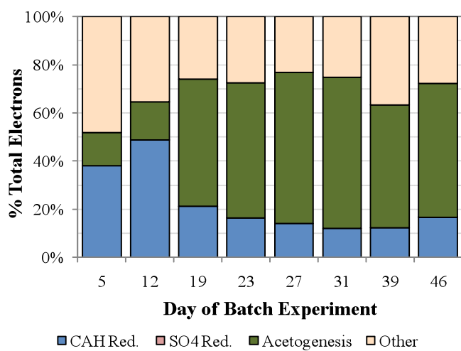
Figure P.13: Electron balance for the PAS-535 reactors
