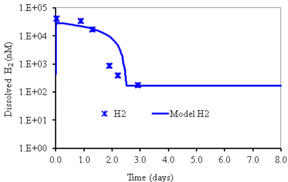
Figure 33 B: Experimental and simulated results of H 2 in batch experiment using cells harvested from the 5-L CSTR. K_{\max} of VC = 26.0 \mu\text{mol/mg protein-d} and K_s = 12 \mu\text{mol/L} .
