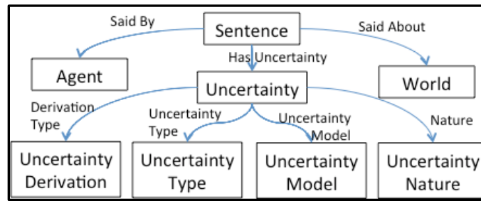
Figure 6 – Uncertainty Ontology
