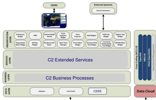
Figure 9 C2 Data-Synchronization Services (C2SS)
