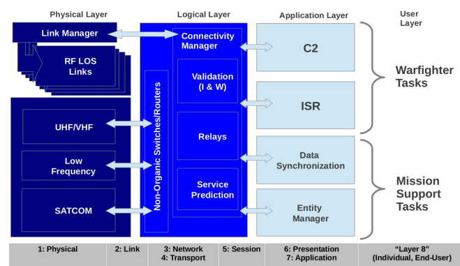
Figure 12 Systems View of RF LOS Link-Management
