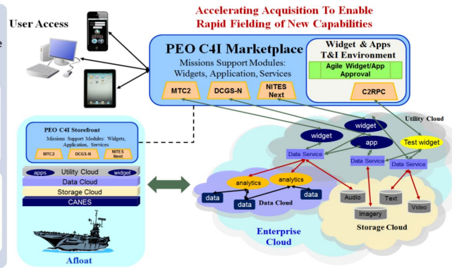
Figure 18 Example of A Model for Reusable UxS Widgets within EA/SOA/Cloud Frameworks
