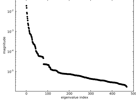
Figure 7.1: Spectrum of the inverted nos5 stiffness matrix.
