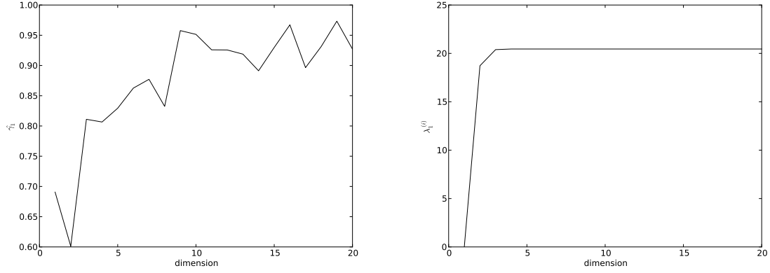
Figure 6.7: Values of \hat{\gamma}_i / \hat{\gamma}_{i+1} (left) and \lambda_1^{(n)} (right) for the inverted Colorado road network Laplacian.
