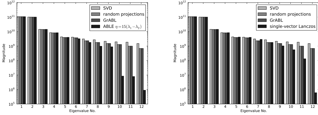
Figure 6.4: Ritz values from minimal 12-dimensional subspaces for GrABL, Lanczos, ABL and random projections.
