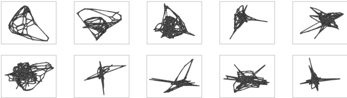
Figure 4.18: Grand tour of first 20 dimensions of commute-time embedding of low-rank approximation of the Colorado Road network graph using the truncated spectral decomposition.
