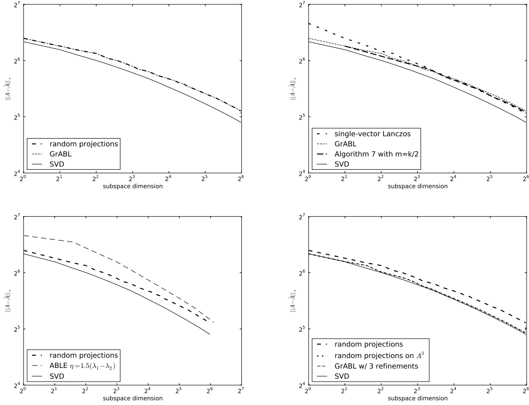
Figure 6.8: Low-rank approximation errors of Colorado graph Laplacian; GrABL v. random projections (top left); GrABL v. single-vector (top right), ABL v. random projections (bottom left) and GrABL v. random projections with refinements (bottom right).
