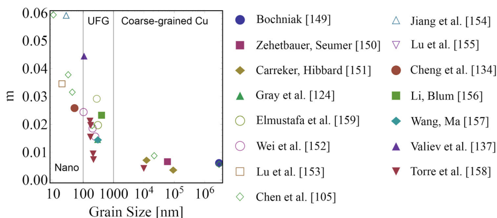
Fig. 10. The strain-rate sensitivity m increases with decreasing grain size for copper processed by a number of different methods. The different grain sizes are categorized into nanocrystalline ( < 100 nm), ultrafine grained (100 nm to 1\mu\text{m} ), and coarse grained ( > 1\mu\text{m} ) for various studies 108,126,134,137,149–159
