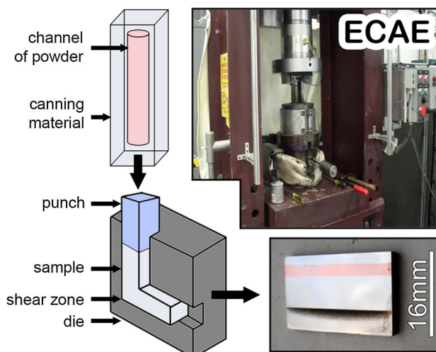
Fig. 4. The equal channel angular extrusion (ECAE) process for consolidation of nanocrystalline powders. The powders are inserted into a canister and heated to an appropriate temperature, and processed using a particular ECAE processing route to fully consolidate the powder material.
