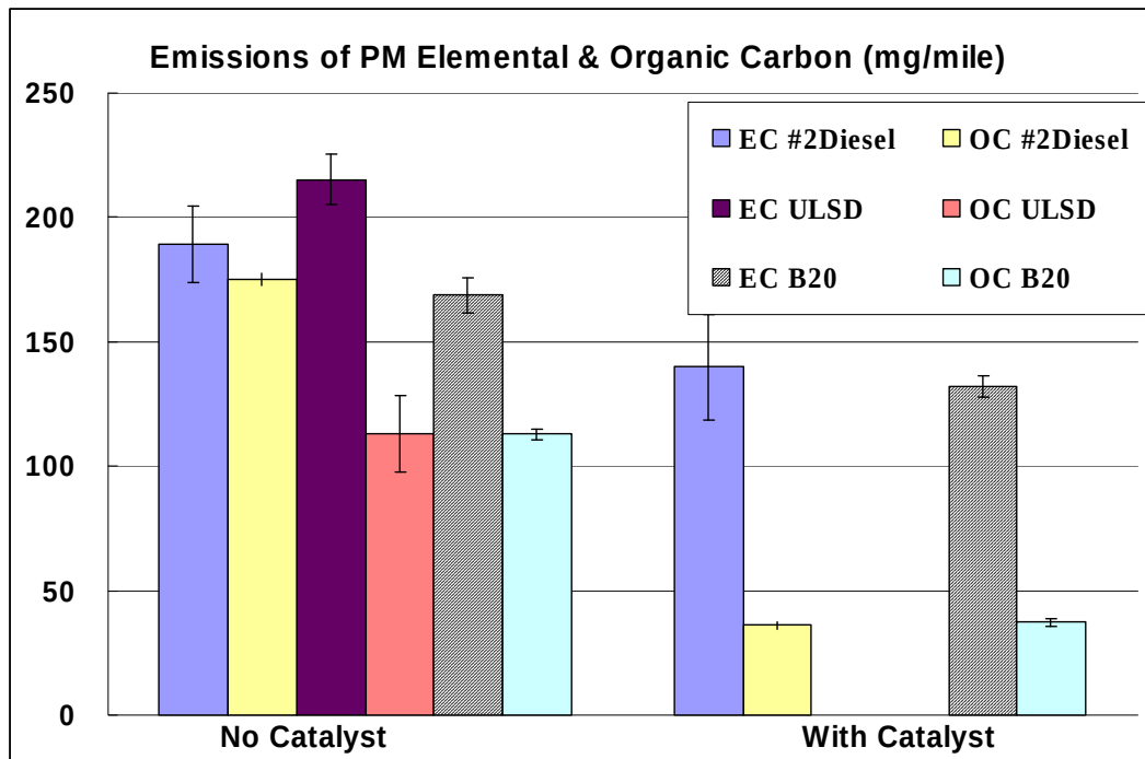
Figure 4. URC Results for Elemental and Organic Carbon for the Cheyenne Mountain Operating Cycle.
