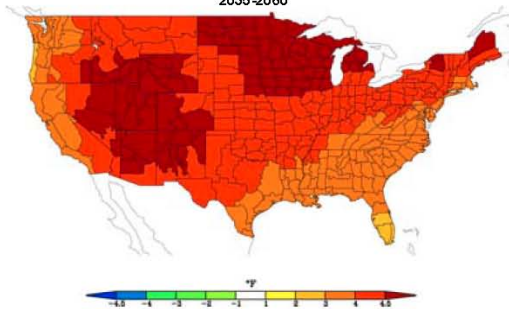
Change in Annual Temperature 2035-2060
