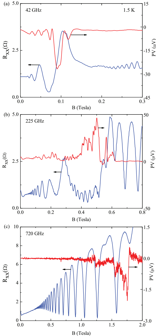
FIG. 4. (Color online) (a) Microwave-induced magnetoresistance oscillations in R_{xx} at f = 42 GHz are shown on the left ordinate. The concurrently measured photo-voltage (PV) is shown on the right ordinate. The PV shows a large and broad feature in the vicinity of the node of the R_{xx} oscillations at B = 0.1 T. (b) R_{xx} (left-ordinate) and PV (right ordinate) at f = 225 GHz. (c) R_{xx} (left-ordinate) and PV (right ordinate) at f = 720 GHz. The largest features in the PV in panels (a) - (c) are associated with cyclotron resonance.
