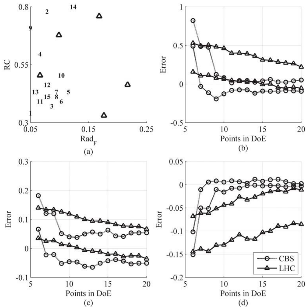
Figure 65: Sampling For Required POI of 1% (a) & 95% Prediction Error Quantiles for Cases of Interest at (b) Mach 0.3, (c) Mach 0.8, and (d) Mach 2.5
