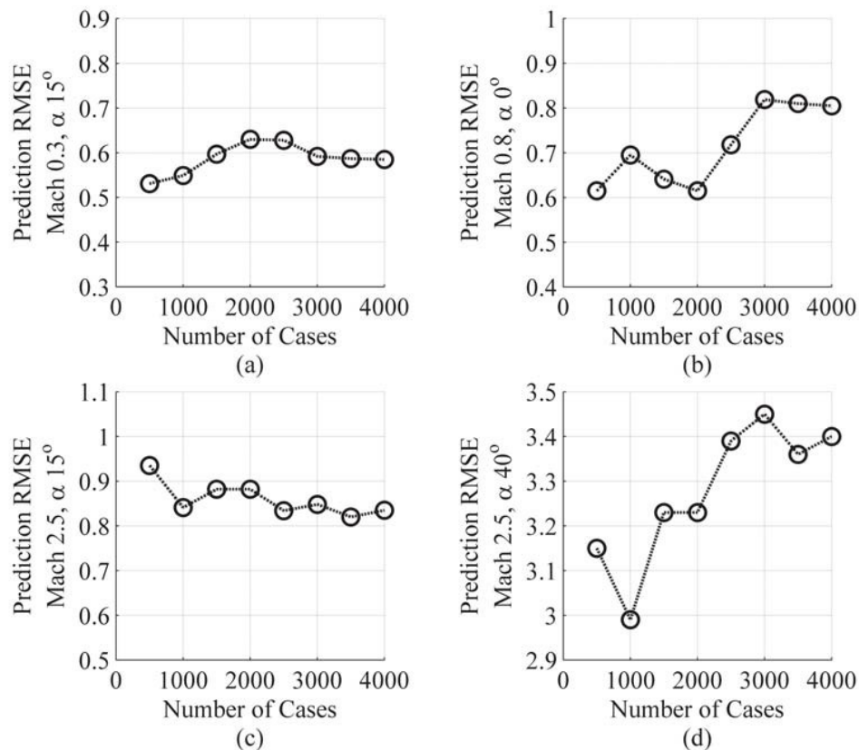
Figure 46: Prediction RMSE for Stacked Latin Hypercube Sampling
