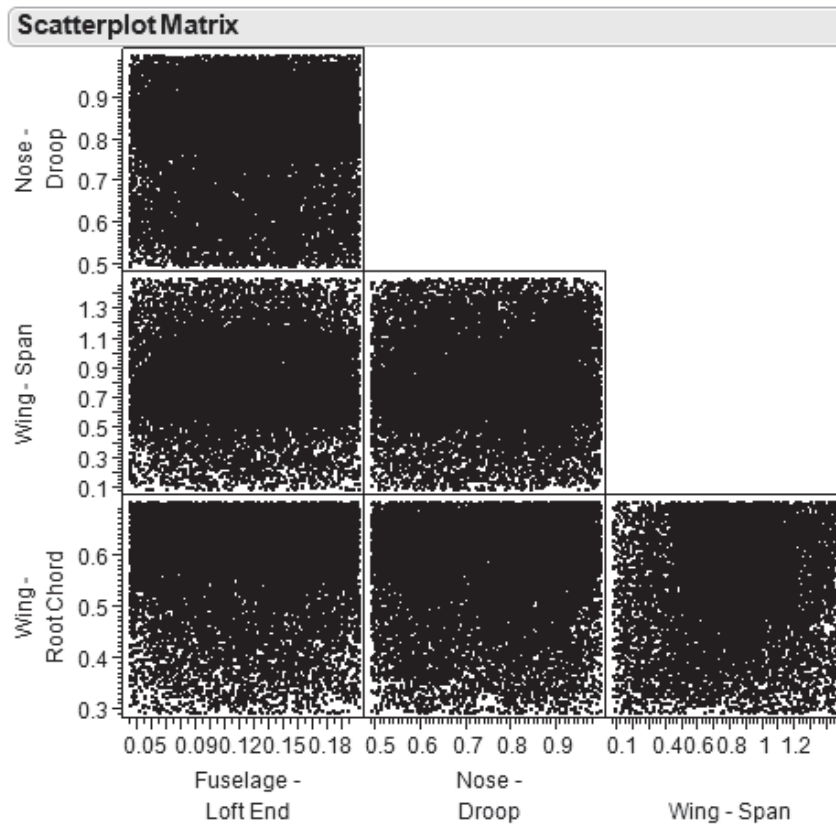
Figure 43: Partial Scatterplot for All Evaluated Cases
