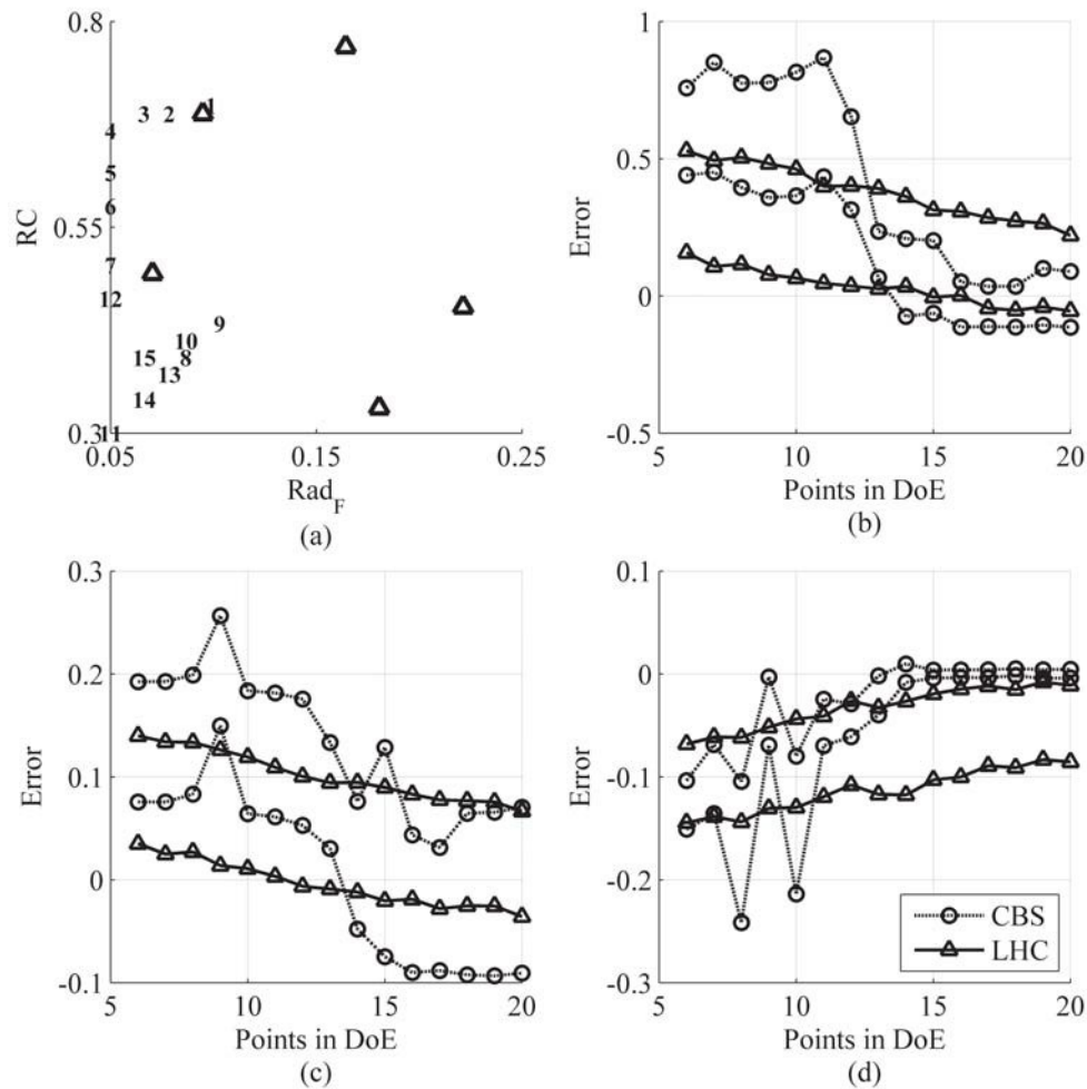
Figure 68: Sampling For Required POI of 15% (a) & 95% Prediction Error Quantiles for Cases of Interest at (b) Mach 0.3, (c) Mach 0.8, and (d) Mach 2.5
