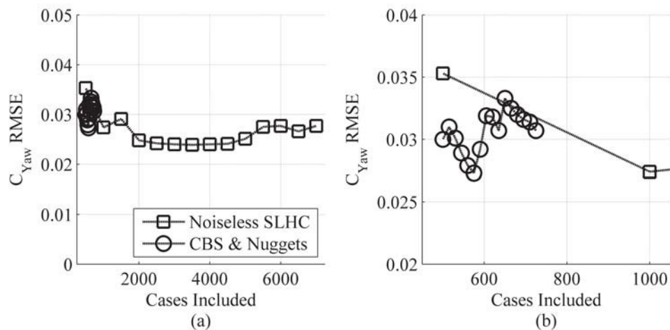
Figure 56: Predictive Accuracy for Yawing Moment at Mach 0.3, \alpha 15^\circ
