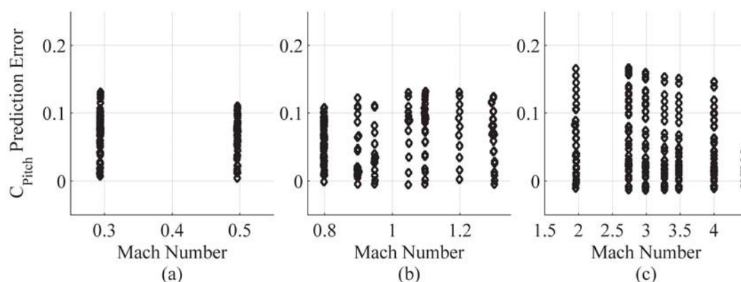
Figure 29: Comparison of Cart3D Results to Wind Tunnel Data, Grouped by Mach Number
