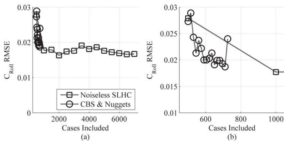
Figure 54: Predictive Accuracy for Rolling Moment at Mach 2.5, \alpha 15^\circ
