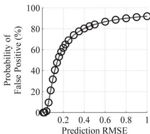
Figure 47: Probability of a False Positive for |C_M| < 0.1
