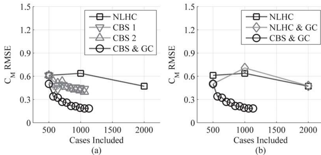
Figure 40: Prediction RMSE at Mach 0.8, \alpha 0^\circ
