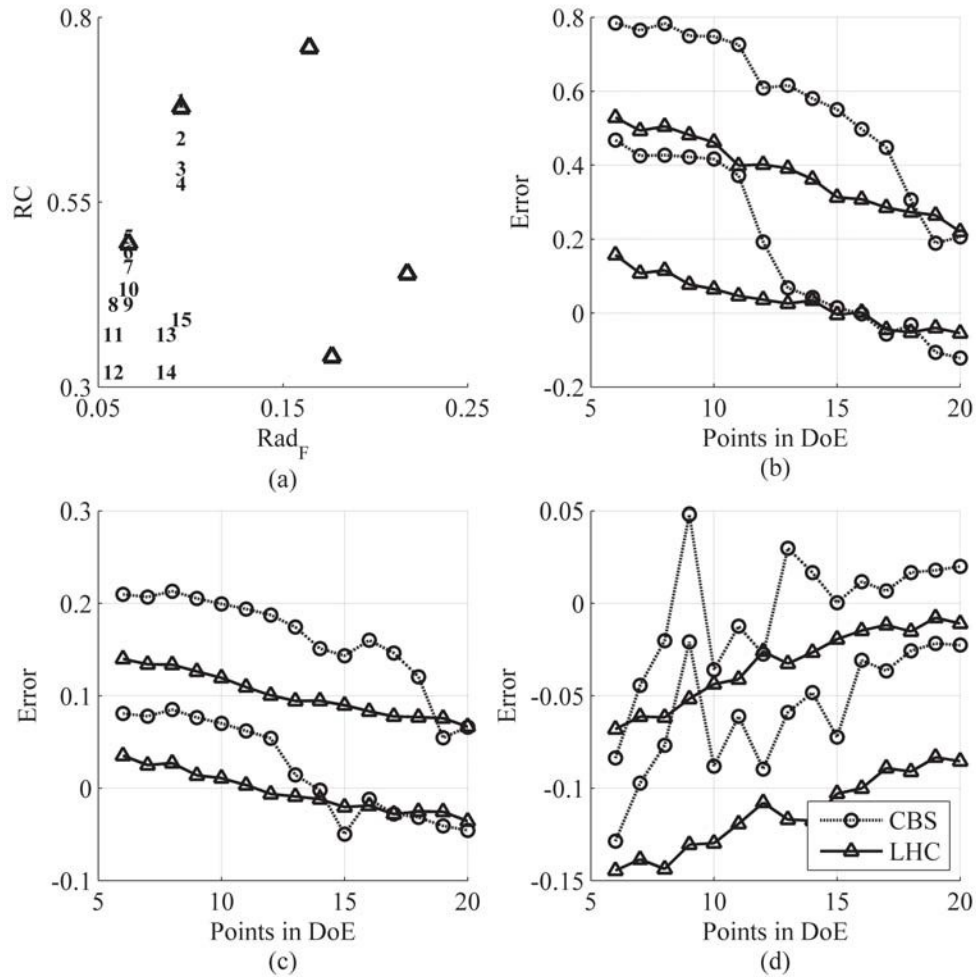
Figure 69: Sampling For Required POI of 25% (a) & 95% Prediction Error Quantiles for Cases of Interest at (b) Mach 0.3, (c) Mach 0.8, and (d) Mach 2.5
