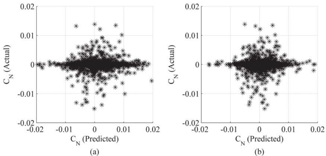
Figure 38: Actual-By-Predicted Plots for Yaw at Mach 4, AoA 40° For (a) a Deterministic Model, and (b) a Model Incorporating Iteration Noise
