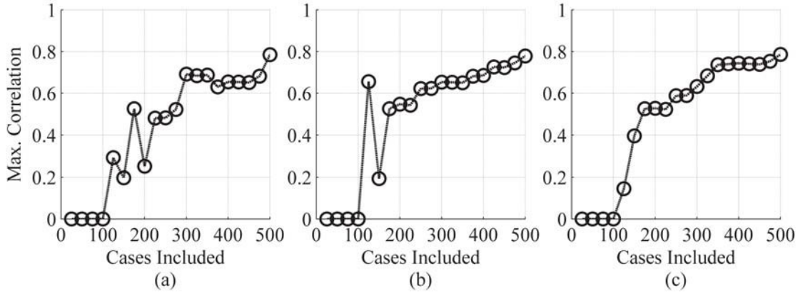
Figure 61: Maximum Correlation Between Any Training Case & Any Test Case
