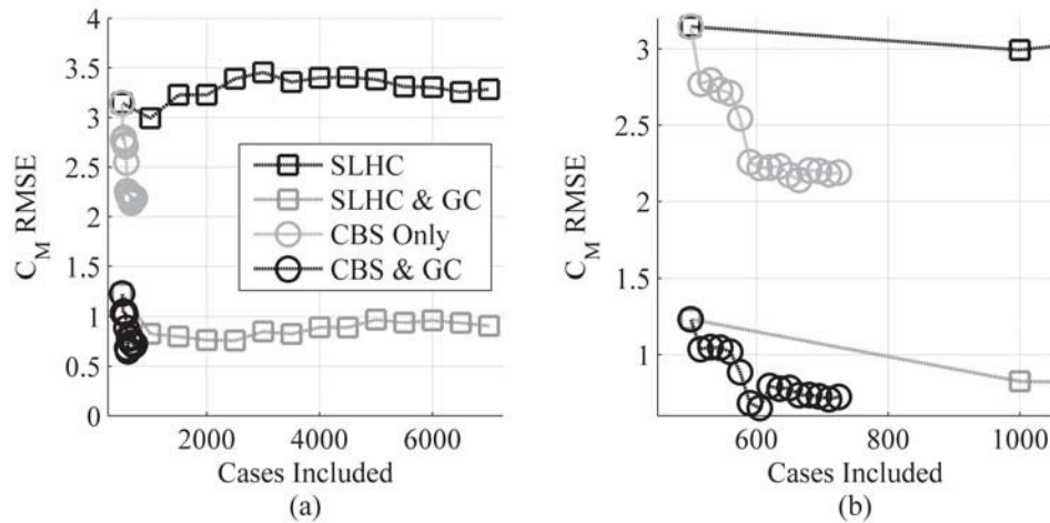
Figure 51: Predictive Accuracy for Pitching Moment at Mach 2.5, \alpha 40°
