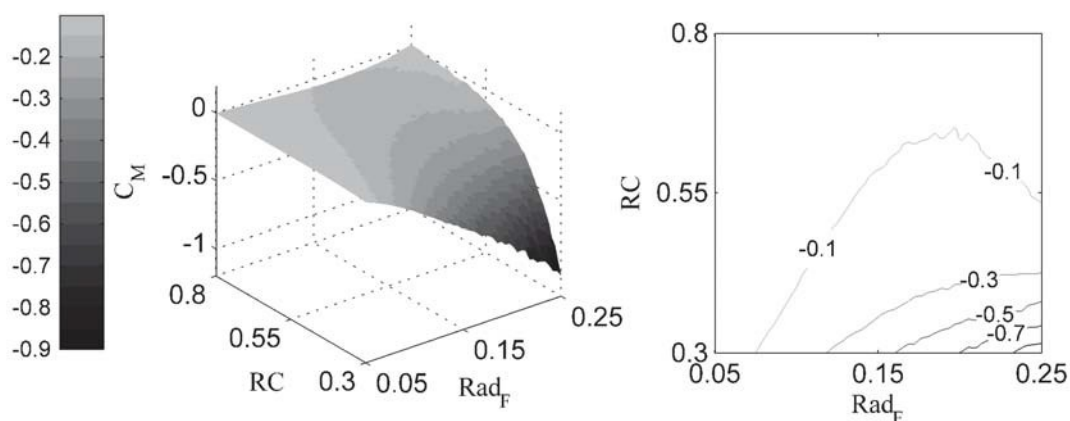
Figure 9: Pitching Moment Coefficient at Mach 2.5, \alpha 0°
