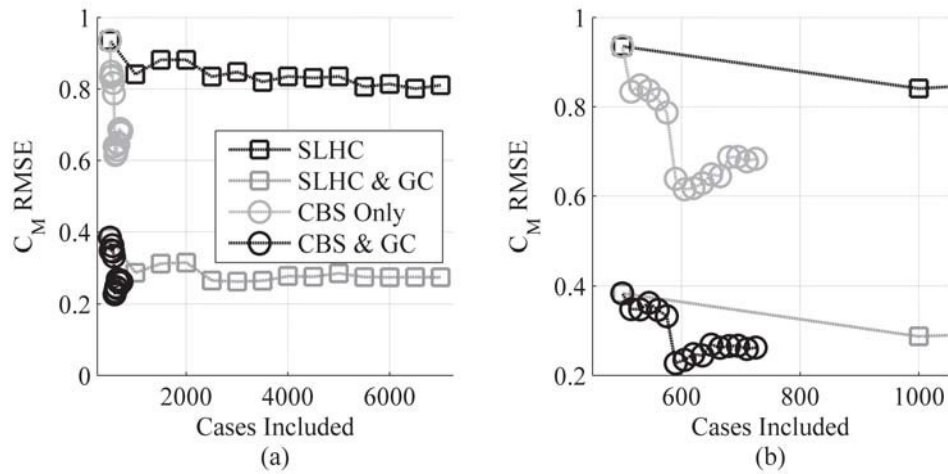
Figure 50: Predictive Accuracy for Pitching Moment at Mach 2.5, \alpha 15°
