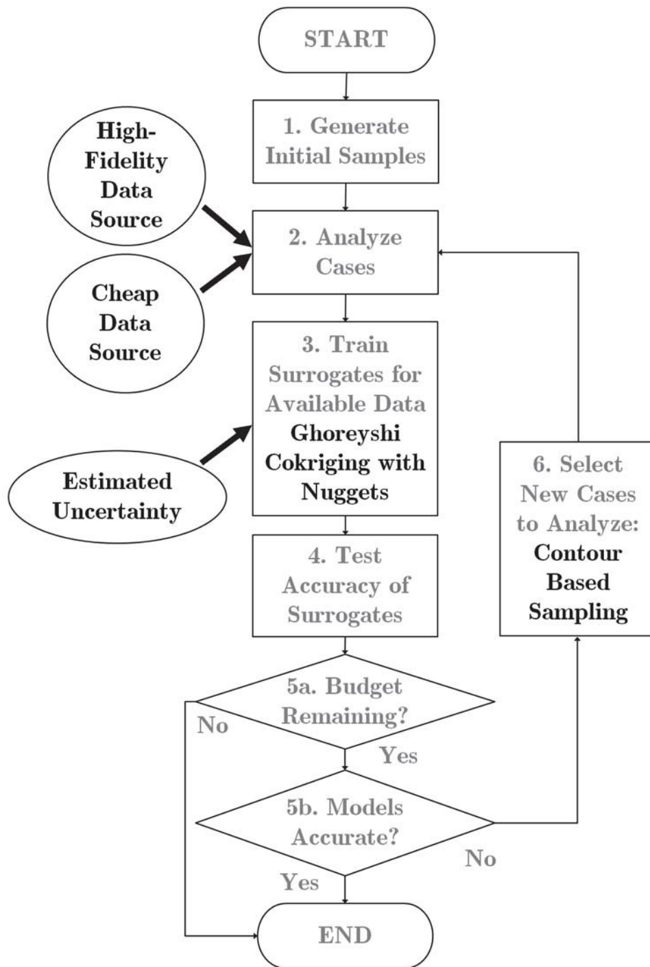
Figure 63: Updated Methodology for Sample Selection & Surrogate Model Creation
