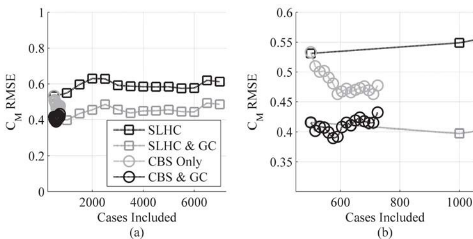
Figure 48: Predictive Accuracy for Pitching Moment at Mach 0.3, \alpha 15°
