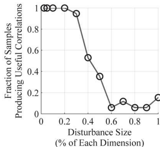
Figure 62: Fraction of Samples That Led To Useful Correlation Coefficients
