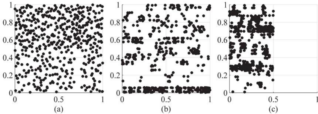
Figure 45: Distribution of Points from Sobol Sequences
