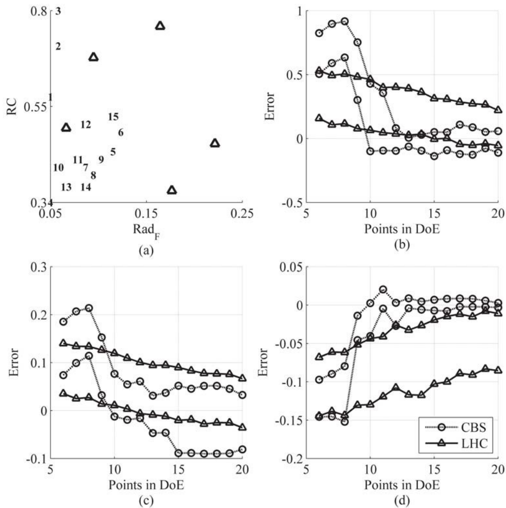
Figure 66: Sampling For Required POI of 5% (a) & 95% Prediction Error Quantiles for Cases of Interest at (b) Mach 0.3, (c) Mach 0.8, and (d) Mach 2.5
