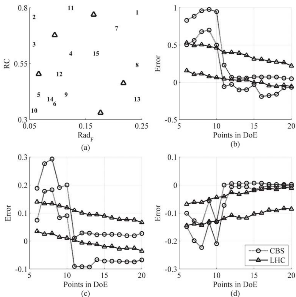
Figure 64: Sampling For Required POI of 0% (a) & 95% Prediction Error Quantiles for Cases of Interest at (b) Mach 0.3, (c) Mach 0.8, and (d) Mach 2.5
