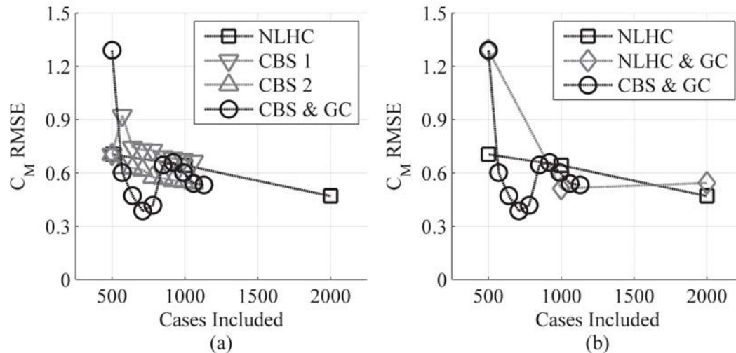
Figure 39: Prediction RMSE at Mach 0.3, \alpha 15°
