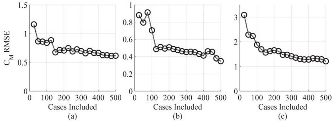
Figure 60: Change in Predictive Accuracy as Training Set Grows
