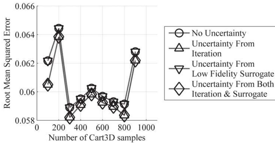
Figure 37: Ghoreyshi Cokriging Prediction RMSE for Yaw at Mach 4, AoA 40°
