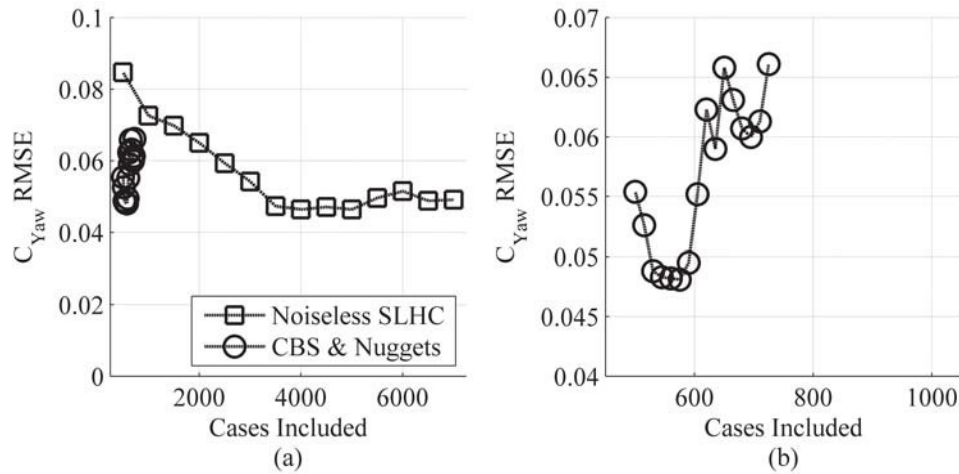
Figure 57: Predictive Accuracy for Yawing Moment at Mach 0.8, \alpha 0^\circ
