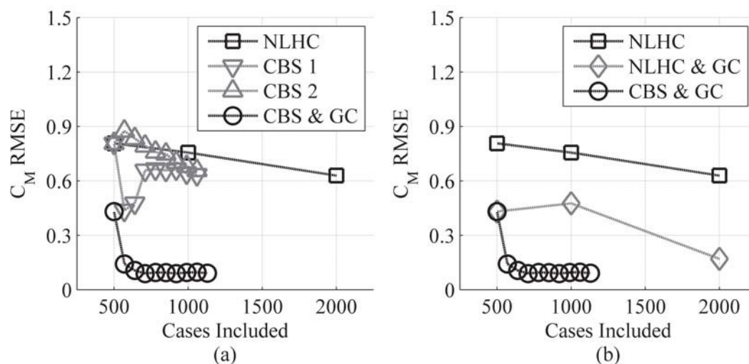
Figure 41: Prediction RMSE at Mach 2.5, \alpha 0°
