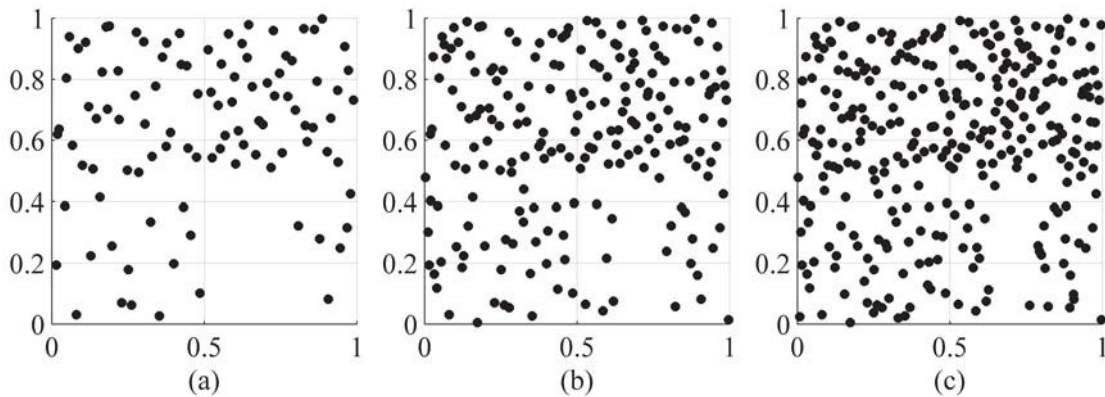
Figure 44: Subsets of a Sobol Sequence
