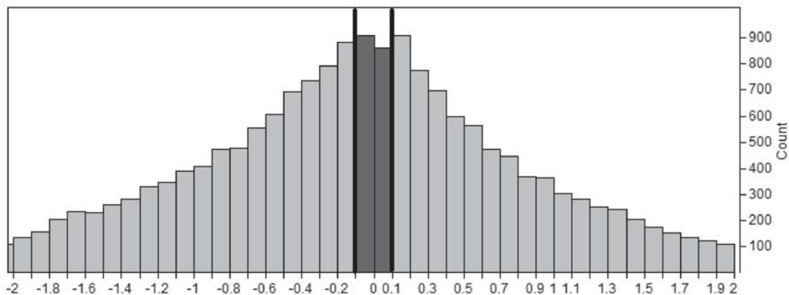
Figure 5: Partial Distribution of Pitching Moments at Mach 0.5, \alpha 0°, \beta 0°
