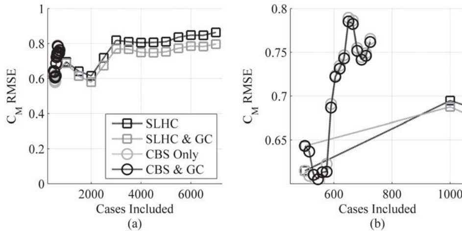
Figure 49: Predictive Accuracy for Pitching Moment at Mach 0.8, \alpha 0°
