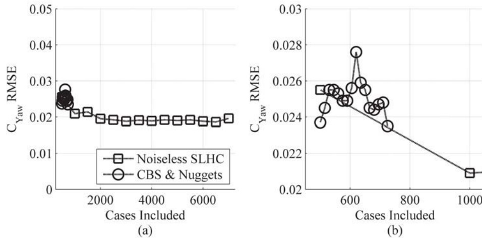
Figure 58: Predictive Accuracy for Yawing Moment at Mach 2.5, \alpha 15^\circ
