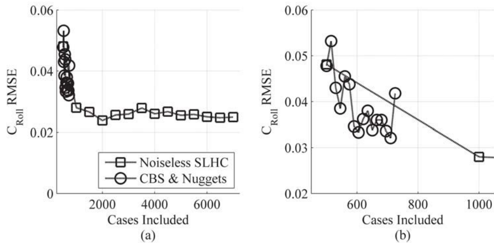
Figure 55: Predictive Accuracy for Rolling Moment at Mach 2.5, \alpha 40^\circ
