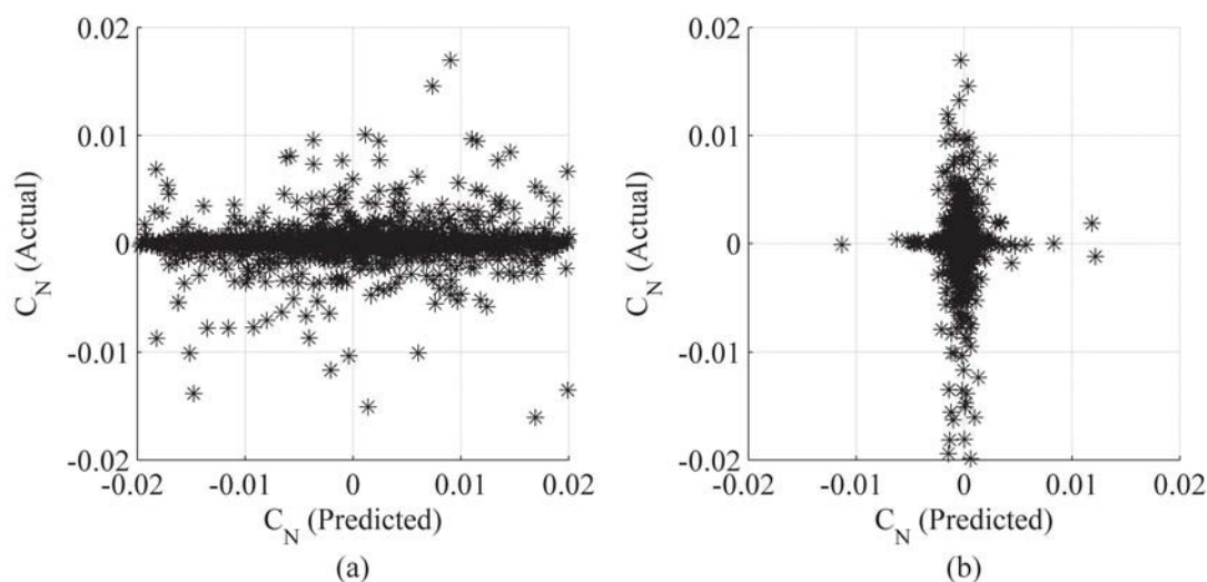
Figure 36: Actual-By-Predicted Plots for Yaw at Mach 4, AoA 0° For (a) Noiseless Model, and (b) Model Incorporating Iteration Noise
