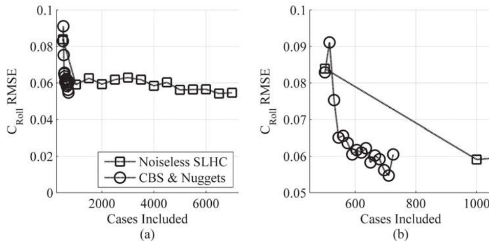
Figure 53: Predictive Accuracy for Rolling Moment at Mach 0.8, \alpha 0^\circ
