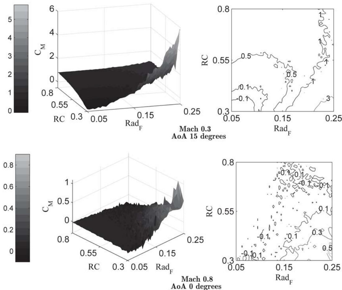
Figure 20: Pitching Moment Coefficient at Mach 0.3, \alpha 15° and Mach 0.8, \alpha 0°
