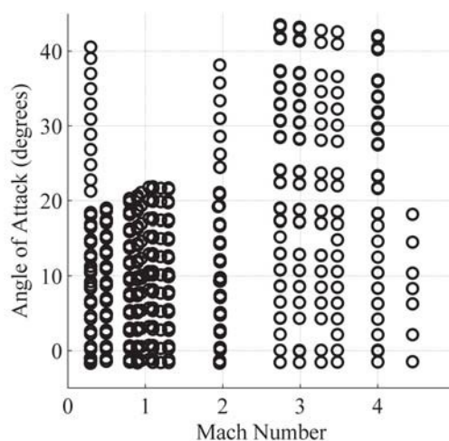
Figure 28: Flight Conditions for XCOR Data
