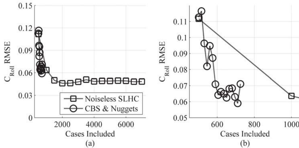
Figure 52: Predictive Accuracy for Rolling Moment at Mach 0.3, \alpha 15^\circ
