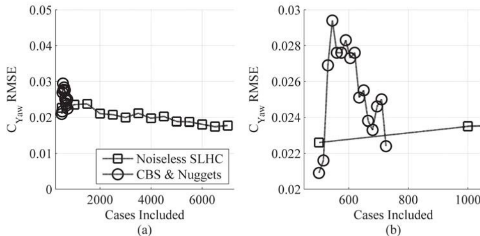
Figure 59: Predictive Accuracy for Yawing Moment at Mach 2.5, \alpha 40^\circ
