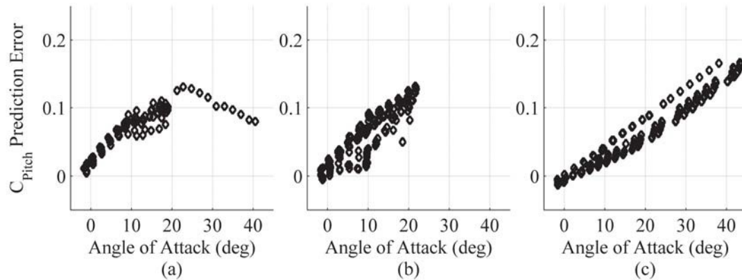
Figure 30: Comparison of Cart3D Results to Wind Tunnel Data, Grouped by AoA for (a) Mach < 0.6; (b) 0.6 < Mach < 1.35; (c) Mach > 1.35
