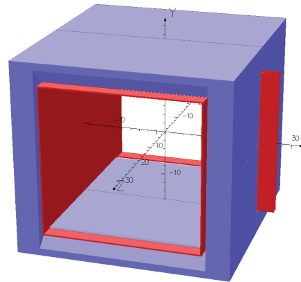
Figure 2. Illustrated magnet structure
