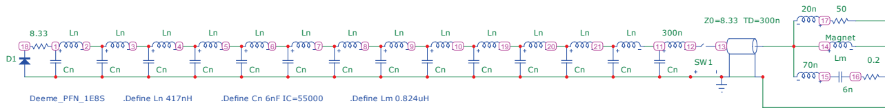
Figure 5. Option 3, an 8.33 ohm impedance kicker system
