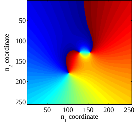
Figure 4.8. The original \phi[\mathbf{n}] plotted for example 2 is shown.
