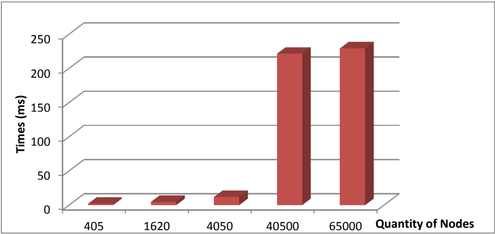
Graphic 2 – Assessment of DijkstraShortestPath Algorithm [8]
