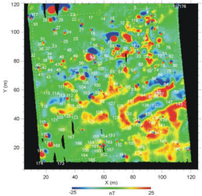
Figure 14. Magnetic Anomalies in Area 2 from Data Collected by the MTADS Vehicular System.
