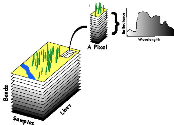
Figure 2. The General Hyperspectral Imaging Concept (measurement of reflected electromagnetic radiation across many tens of contiguous bands where each pixel contains one complete spectral signature used to absolutely identify surface materials).
