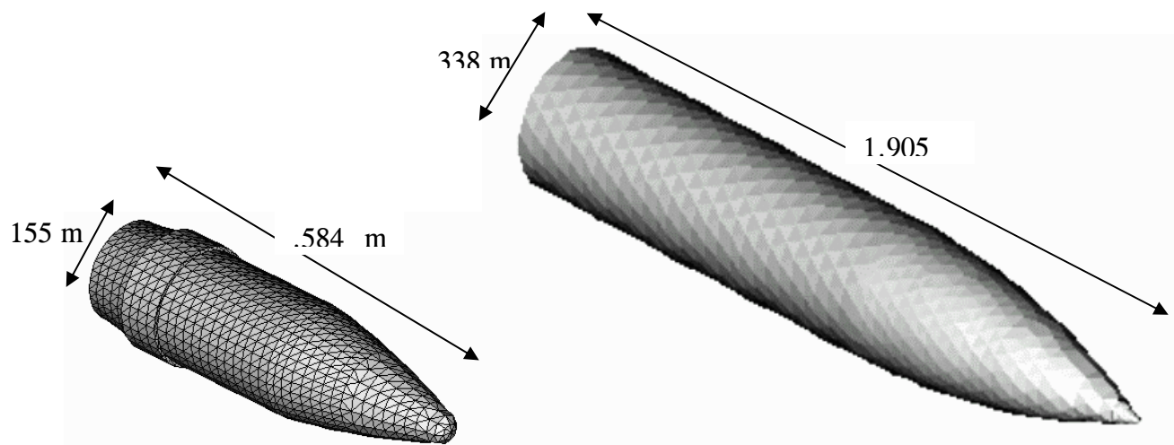
155-mm model (left) and 500-lb bomb model (right)
