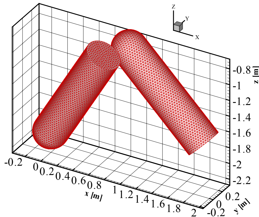
Figure 6. Mesh Used to Model Scattering from Two UXO Buried in Soil. (The soil interface is at z = 0 .)
