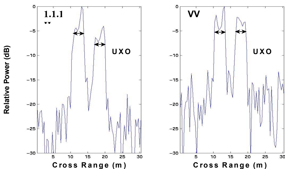
Figure 8. UHF Cross-Range Cut Through UXOs from 0^\circ Aircraft Heading Image, 2,000-lb Bomb Dense Deployment.
