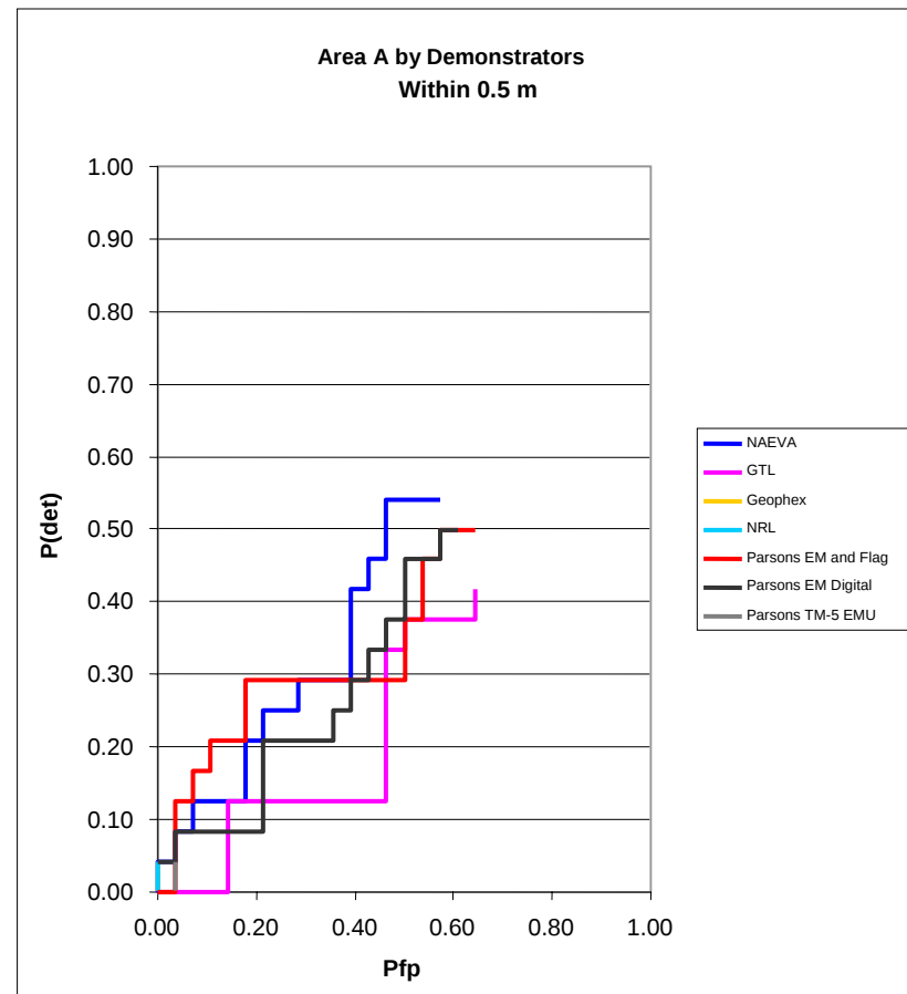
Figure 46. Area A— P(\text{det}) Versus P_{\text{fp}} Within 0.5 m for All Demonstrators.
