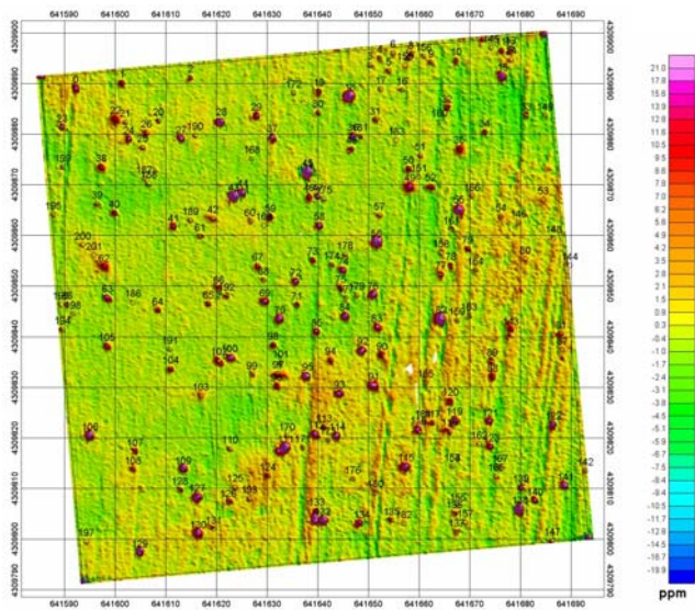
Figure 20. Geopex Ltd. GEM-3 Survey of Area 3.
