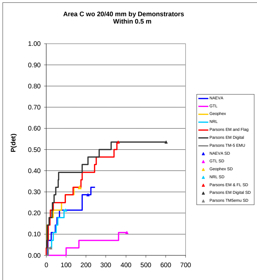
Figure 45. Area C Without 20 and 40 mm— P(\text{det}) Versus Total FAR Within 0.5 m for All Demonstrators.
