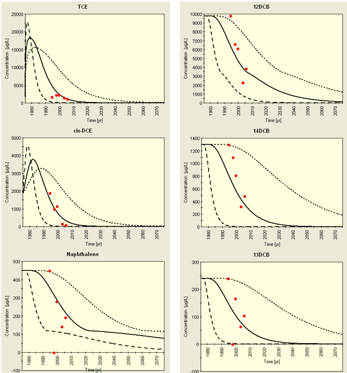
Figure 5. Observed Versus NAS-Simulated Concentrations at a Source-Zone Monitoring Well for Six NAPL Compounds Using a Range of Velocity Estimates.
