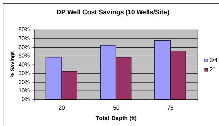
Figure 1. Percentage Savings for DP Well Installations Based on Well Diameter and Depth.
