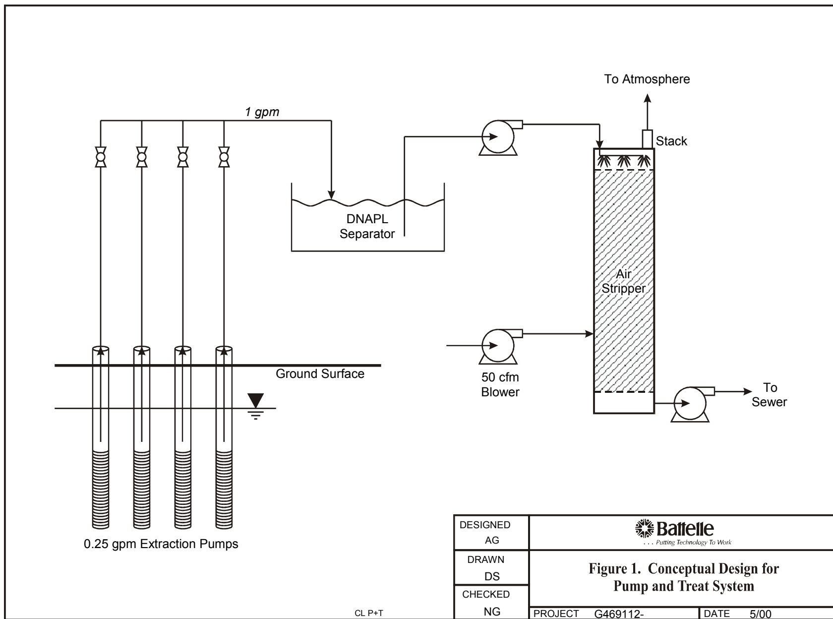
Figure D.1. Conceptual Design for P&T System.
