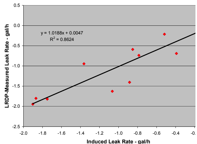
Figure 4. Least-Squares Lines Fitted to the Test Results of the LRDP-24. (Tests conducted with induced leaks are shown in red.)
