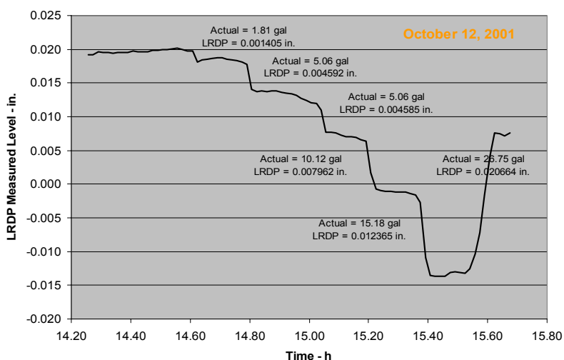
Figure 5. Height-to-Volume Calibration Test Results for the 54-ft-Diameter Fixed-Roof AST with a Floating Pan.
