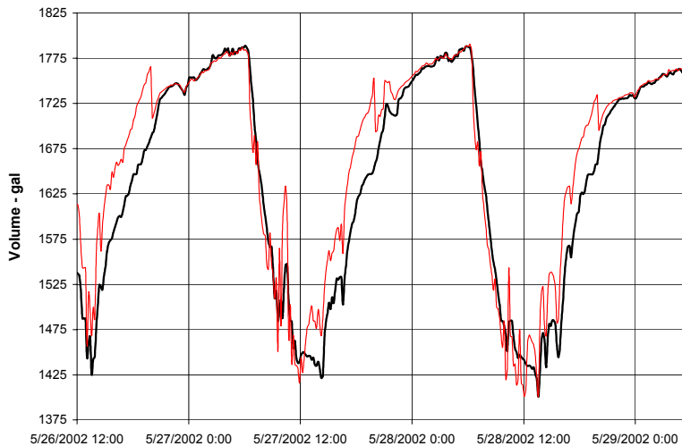
Figure 3. Level and Shell Temperature Data Obtained with the LRDP-24 System During Pre-Evaluation LRDP Tests.
