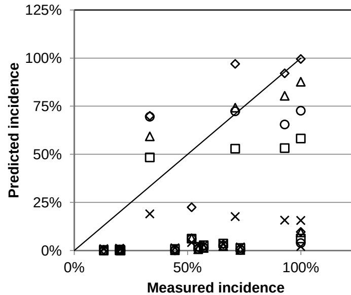
Figure 4. Probability of dive-stopping events during dry hyperbaric exposure, model prediction vs. measured data. \square :H95A, \diamond :H95B, \circ :H93, \Delta :A02A, \times :A02B. The identity line is shown.
