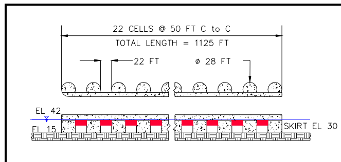
Figure 4. Multicell ported guard wall with skirts
