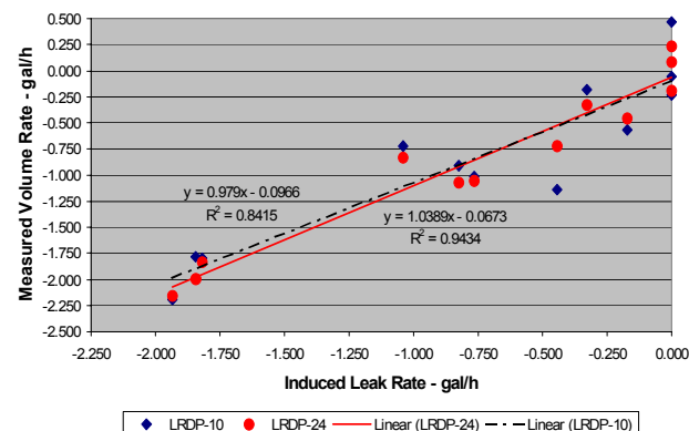
Figure 8. Least-Squares Lines Fitted to the Test Results of the LRDP-10 and the LRDP-24.
