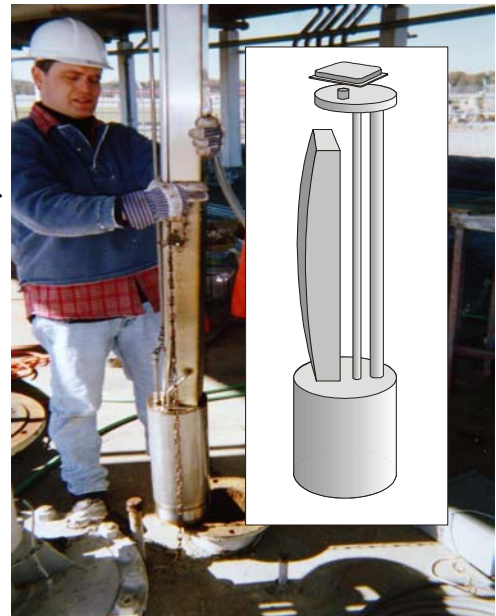
Figure 5. Installation of the LRDP in the 50,000-gal UST at the Hunter Army Airfield.
