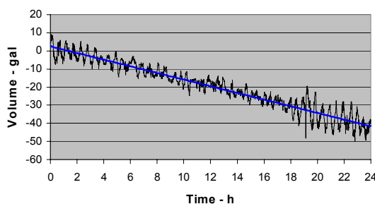
Figure 7. Level Data Obtained with the LRDP-24 System for Test 10.
