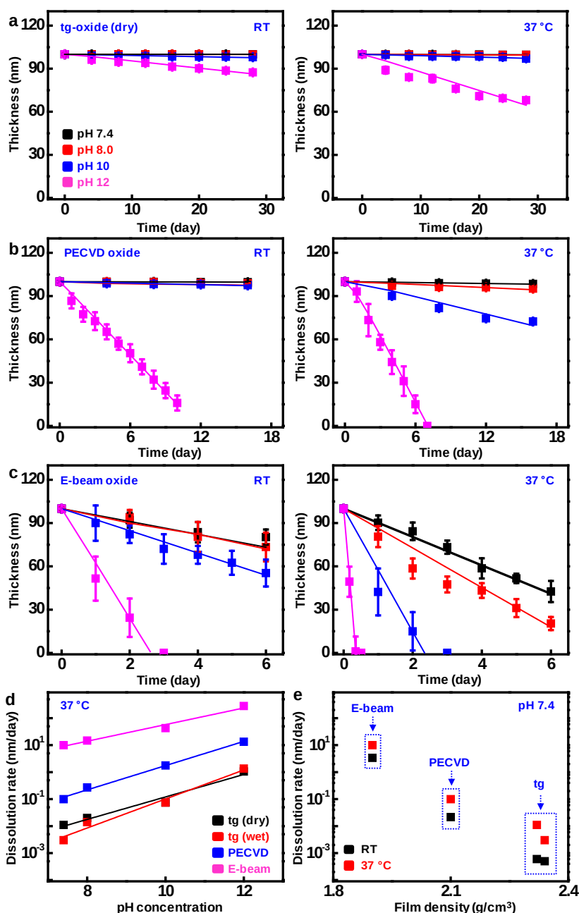
Figure 5: Dissolution Kinetics
