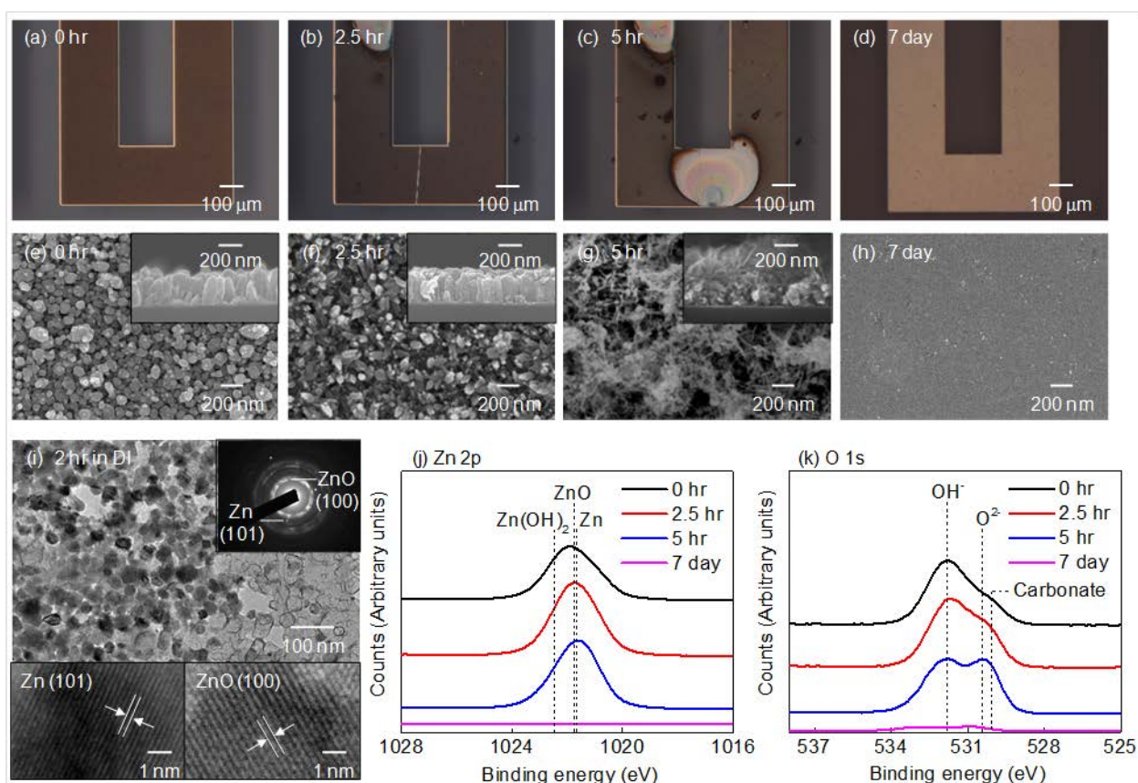
Figure 15: Evolution of Microstructure and Surface Chemistry Associated with Dissolution of Zn in DI Water
