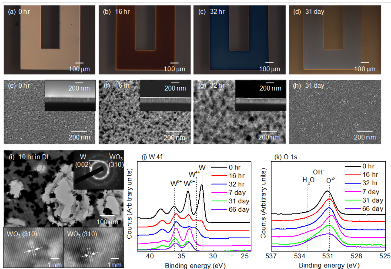
Figure 13: Evolution of Microstructure and Surface Chemistry Associated with Dissolution of Sputtered Deposited W in DI Water (a)-(d) optical images; (e)-(h) SEM images with cross-sectional views in the insets; (i) TEM bright field image with diffraction patterns and lattice fringes; (j)-(k) XPS data.
