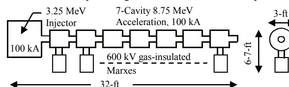
Figure 9. ACLIA schematic.
