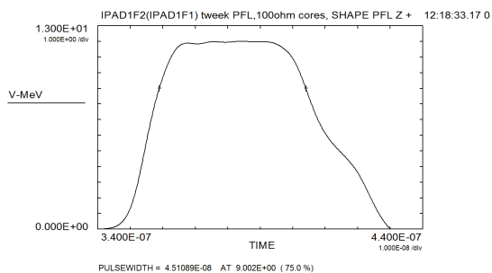
Figure 2. IVA cell voltage waveform.
