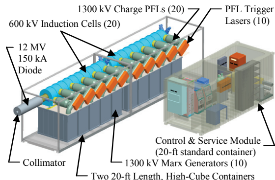
Figure 1. Induction Voltage Adder (IVA).
