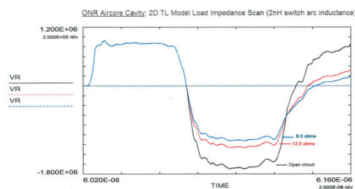
Figure 8. ACLIA cell output from 2-D TL model.
