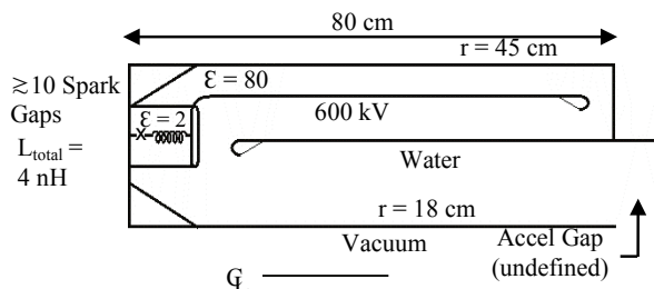
Figure 7. Coaxial ACLIA cell.
