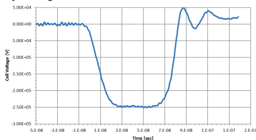
Figure 4. ATA Blumlein waveform.
