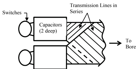
Figure 5. Marxing two LTD bricks.
