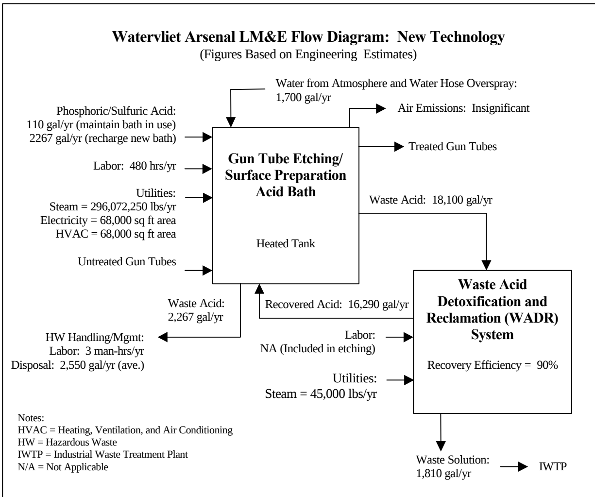
Figure 5. Labor, Material and Energy (LM&E) Balances for WADR Process
