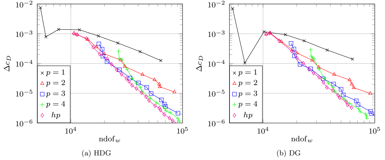
Figure 12: Drag convergence with respect to degrees of freedom ( \text{Ma}_\infty = 0.5 , \alpha = 1^\circ , \text{Re} = 5000 )
