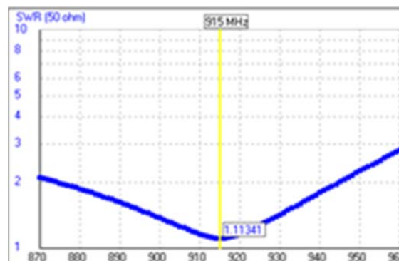
Figure 27. SWR graph of first 915 MHz antenna
