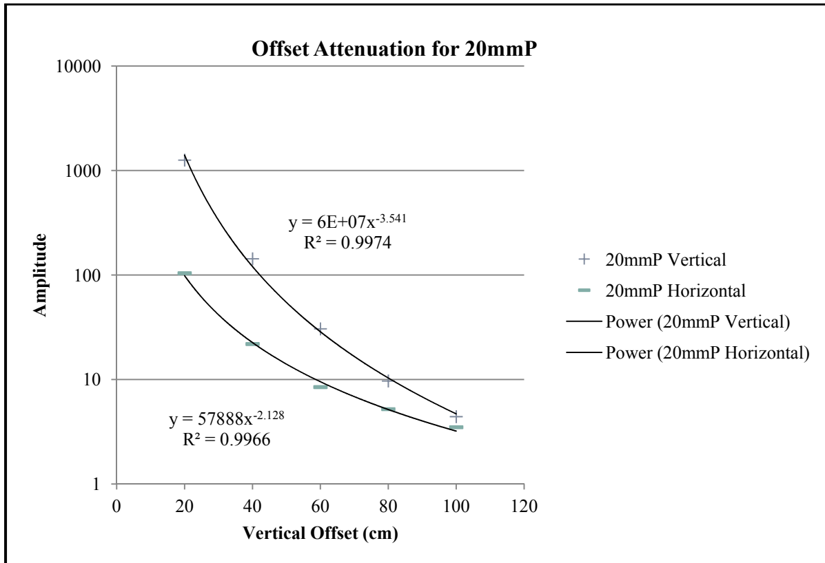
Figure 8: Signal attenuation due to altitude (offset) for a 20mm projectile. Vertical (most favorable) and horizontal (least favorable) orientations are shown. The lowest response amplitude at the maximum depth of 20x diameter (40cm depth, 60cm offset) is approximately 10ppm.
