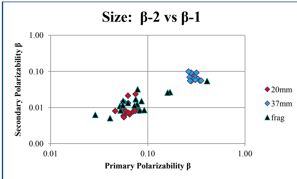
Figure 11: Plot of secondary vs. primary polarizability amplitude for ground truth seeds at West Jefferson Grid.
