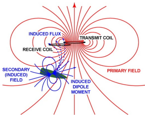
Figure 1: (a-left) Theoretical model of primary and secondary electromagnetic fields. (b-right) Photo of Battelle airborne TEM-8 system.
