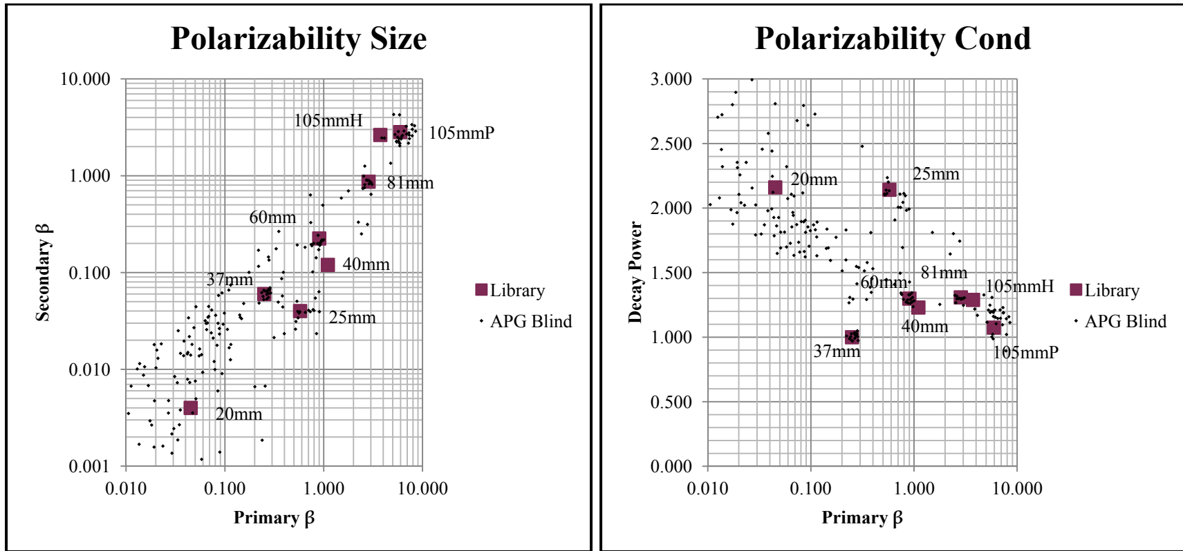
Figure 20: (a-left) Plot of secondary vs. primary polarizability amplitude and (b-right) primary polarizability decay power vs. amplitude. Points include the Library reference points and all detected targets from the APG Blind Grid.
