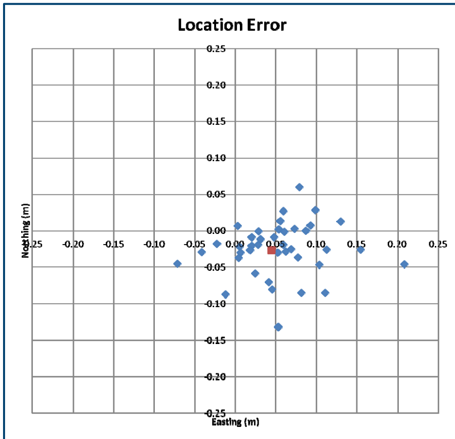
Figure 16: Calibration Grid location error plot. The average offset is shown in red. The standard deviation is 0.05m
