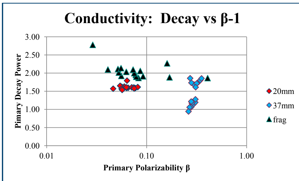
Figure 12: Plot of primary polarizability decay power vs. amplitude for ground truth seeds at West Jefferson Grid.
