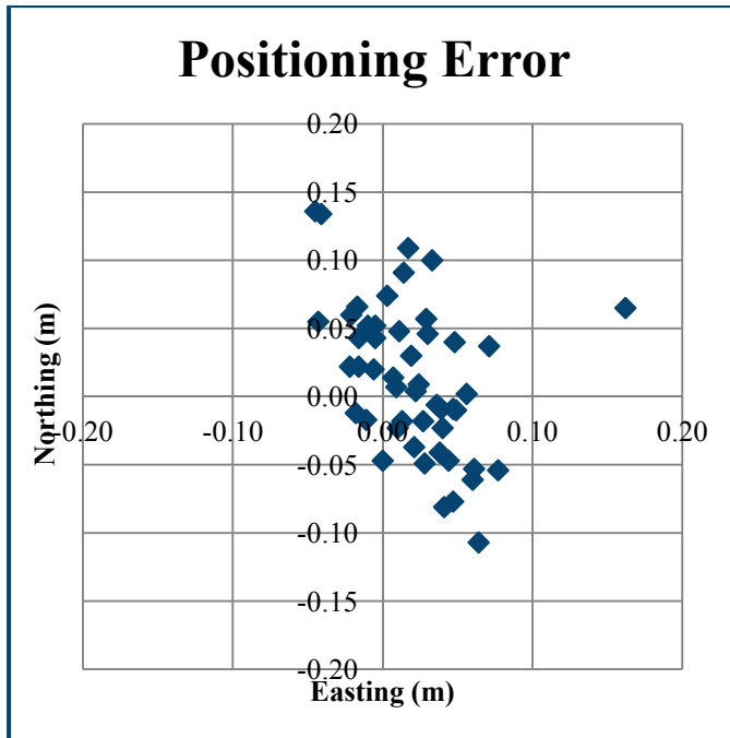
Figure 10: Plot of target location error from the West Jefferson Grid.
