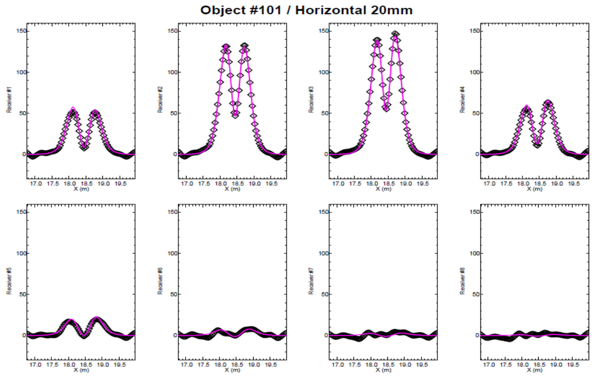
Figure 3: Plots of measured and modeled EM response across the array (receivers 1-8) over vertical and horizontal 20mm targets from Camp Sibert field test.
