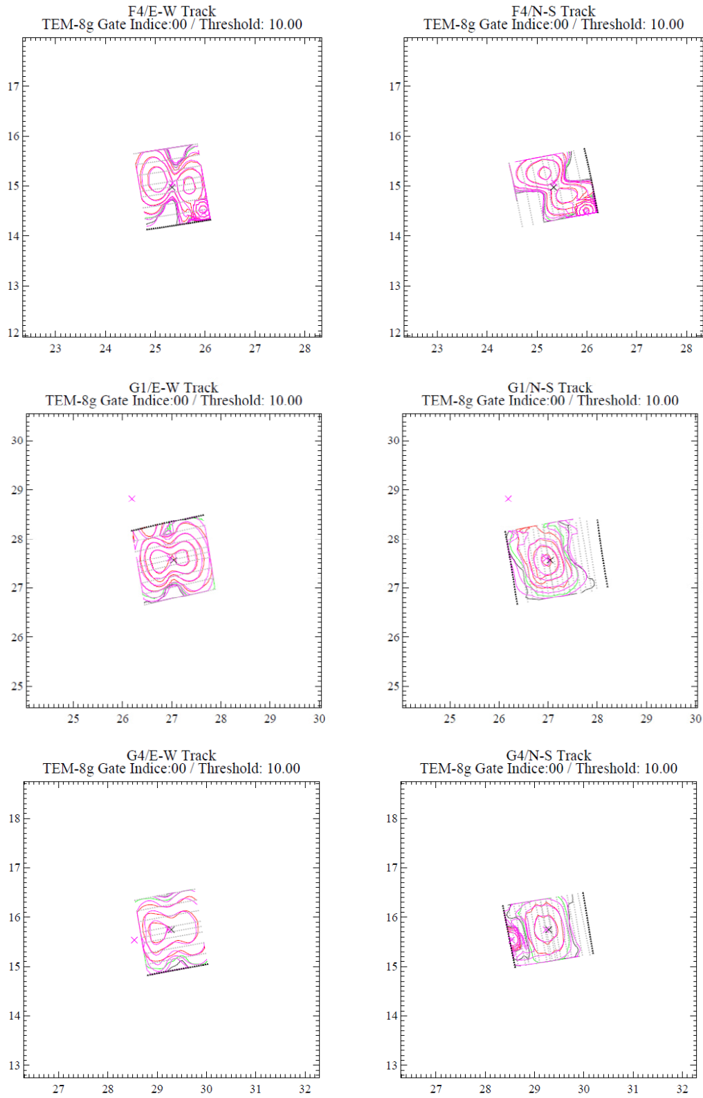
Figure 15: Overlapping contours of measured and modeled (from inverted target) results of 2-dipole models for anomalies in Calibration Grid Cells F4 (25mm), G1 (37mm) and G4 (37mm).
