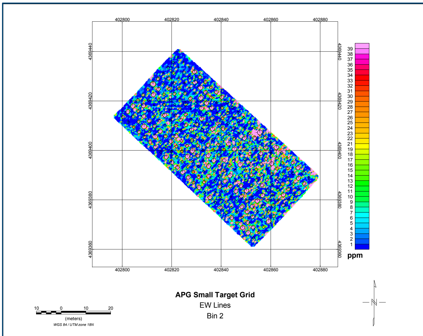
Figure 22: Plot of Bin2 response at APG Calibration Grid after removal of background susceptibility.
