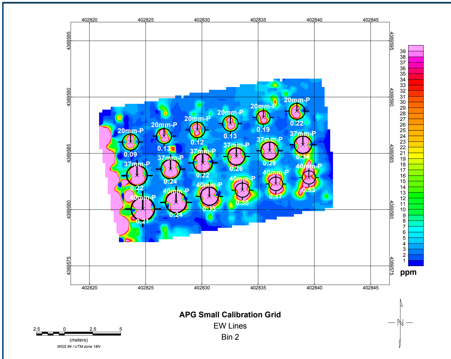
Figure 14: Plot of Bin2 response at APG Calibration Grid.
