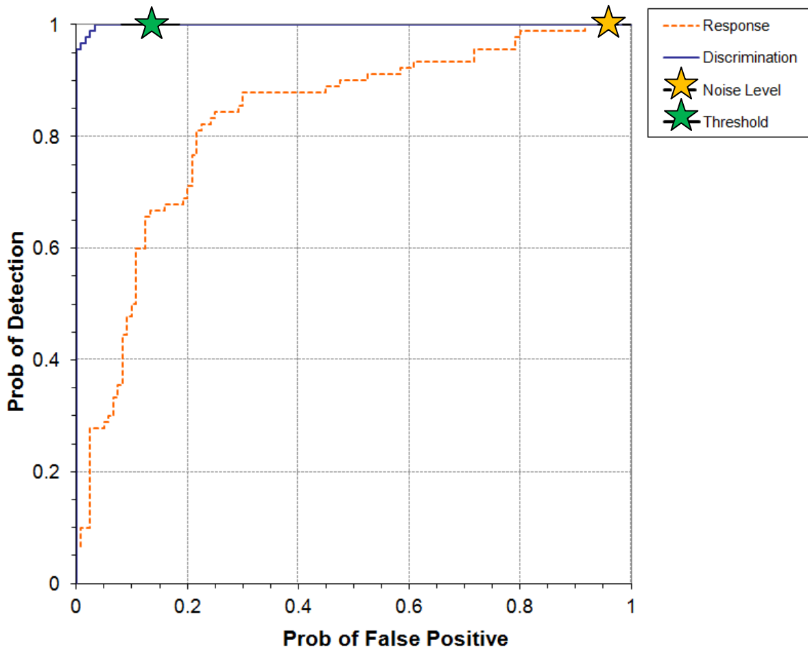
Figure 21: ROC curve for TEM-8g at Blind Grid. Probability of detection for response and discrimination stages versus their respective probability of false positive.
