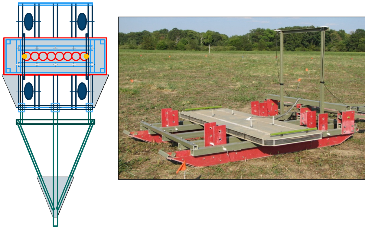
Figure 2: Schematic (a-left) and photo (b-right) of the TEM-8g system. Red lines on schematic show transmitter and receiver coils. Schematic shows wheeled option, photo shows ski option. Sled option not shown.
