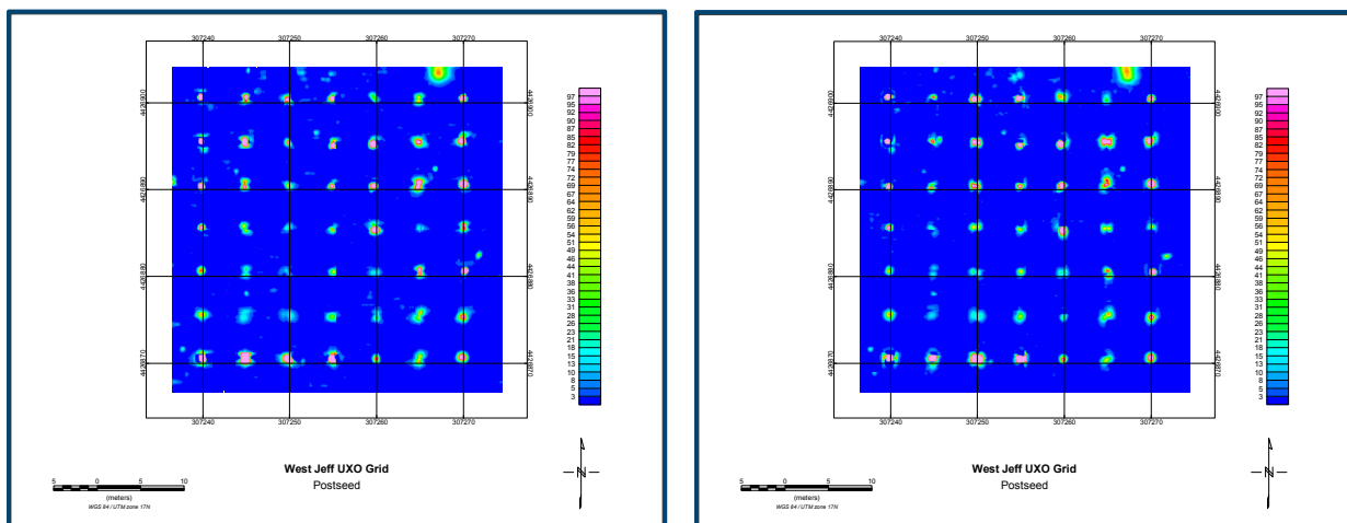
Figure 9: Thumbnail plots of the Bin2 response for the NS (left) and EW (right) survey lines at the West Jefferson Grid. Grid lines are at 10m intervals, color scale is 0-100ppm.
