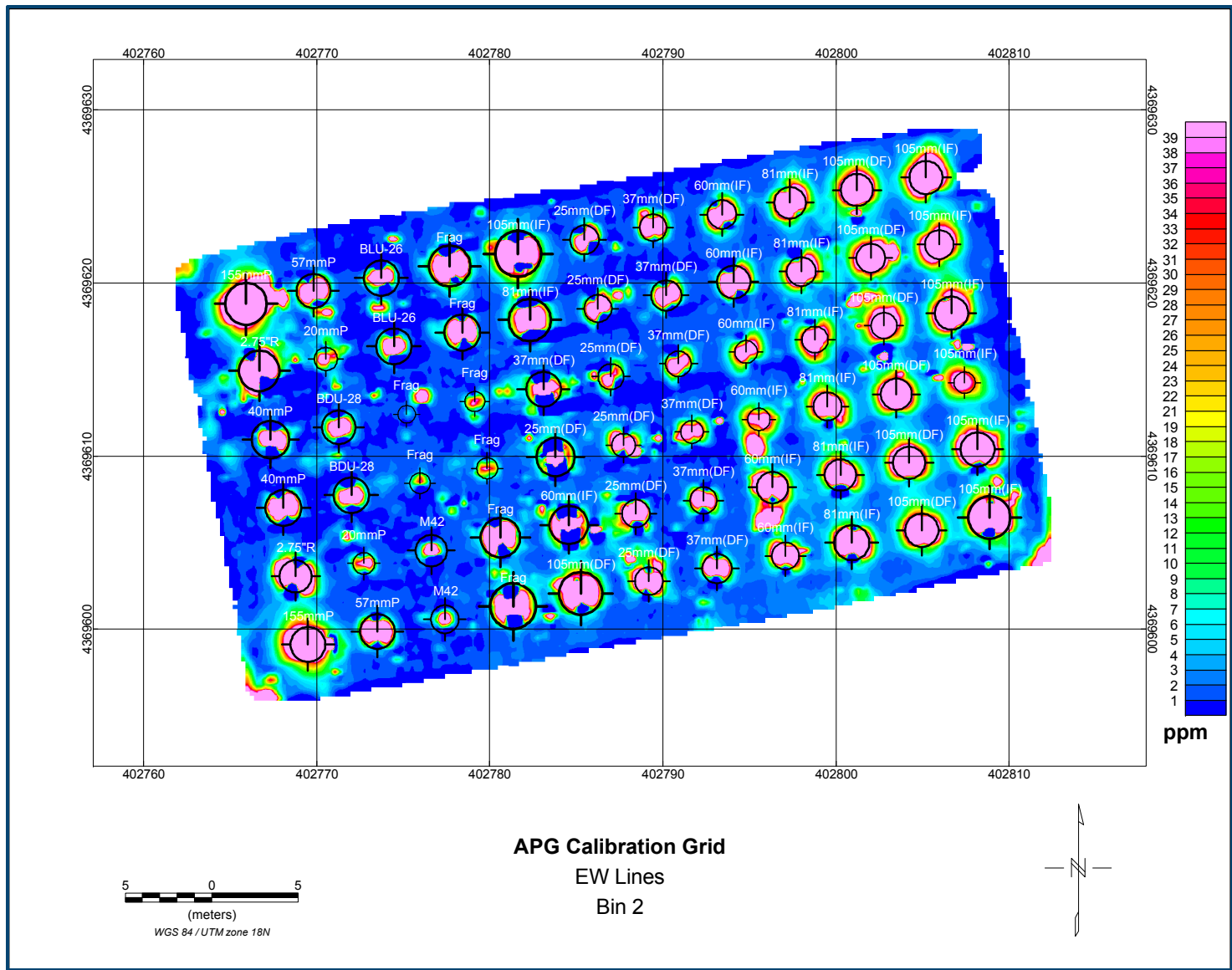
Figure 13: Plot of Bin2 response at APG Calibration Grid.
