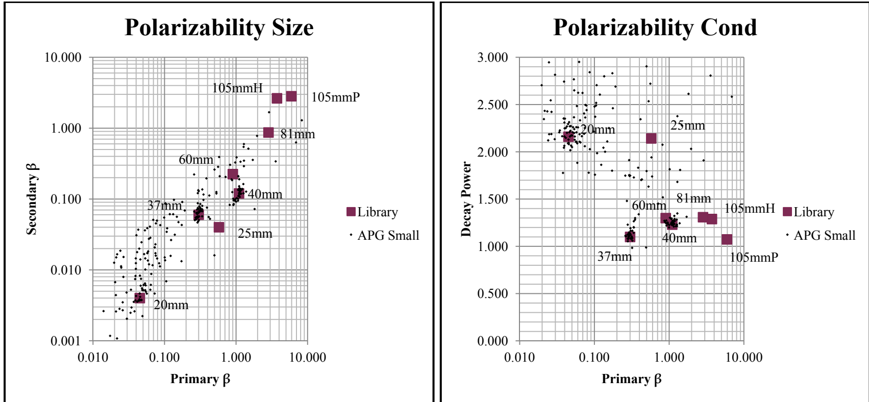
Figure 23: (a-left) Plot of secondary vs. primary polarizability amplitude and (b-right) primary polarizability decay power vs. amplitude. Points include the Library reference points and all detected targets from the APG Small Target Grid. Note that the variant of 20mm projectiles used at the West Jefferson test grid are not represented in this dataset.
