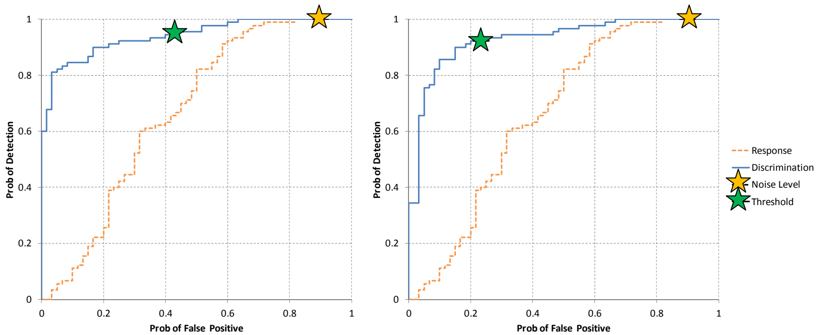
Figure 24: (a-left) ROC curve from Battelle list, Small Target Grid, capped cells, all ordnance types, depths to 20x diameter. (b-right) ROC curve from SAIC list, Small Target Grid, capped cells, all ordnance types, depths to 20x diameter.
