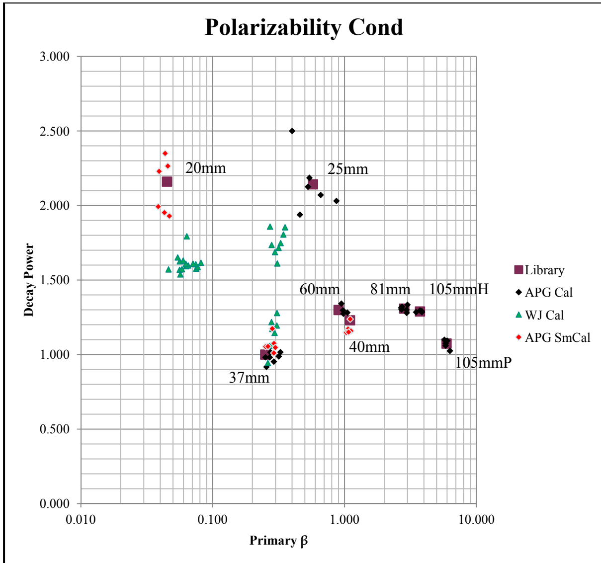
Figure 18: Plot of primary polarizability decay power vs. amplitude for calibration items. Points include individual results from the West Jefferson and APG Calibration grids, as well as the final Library reference point used for classification of the APG grids.
