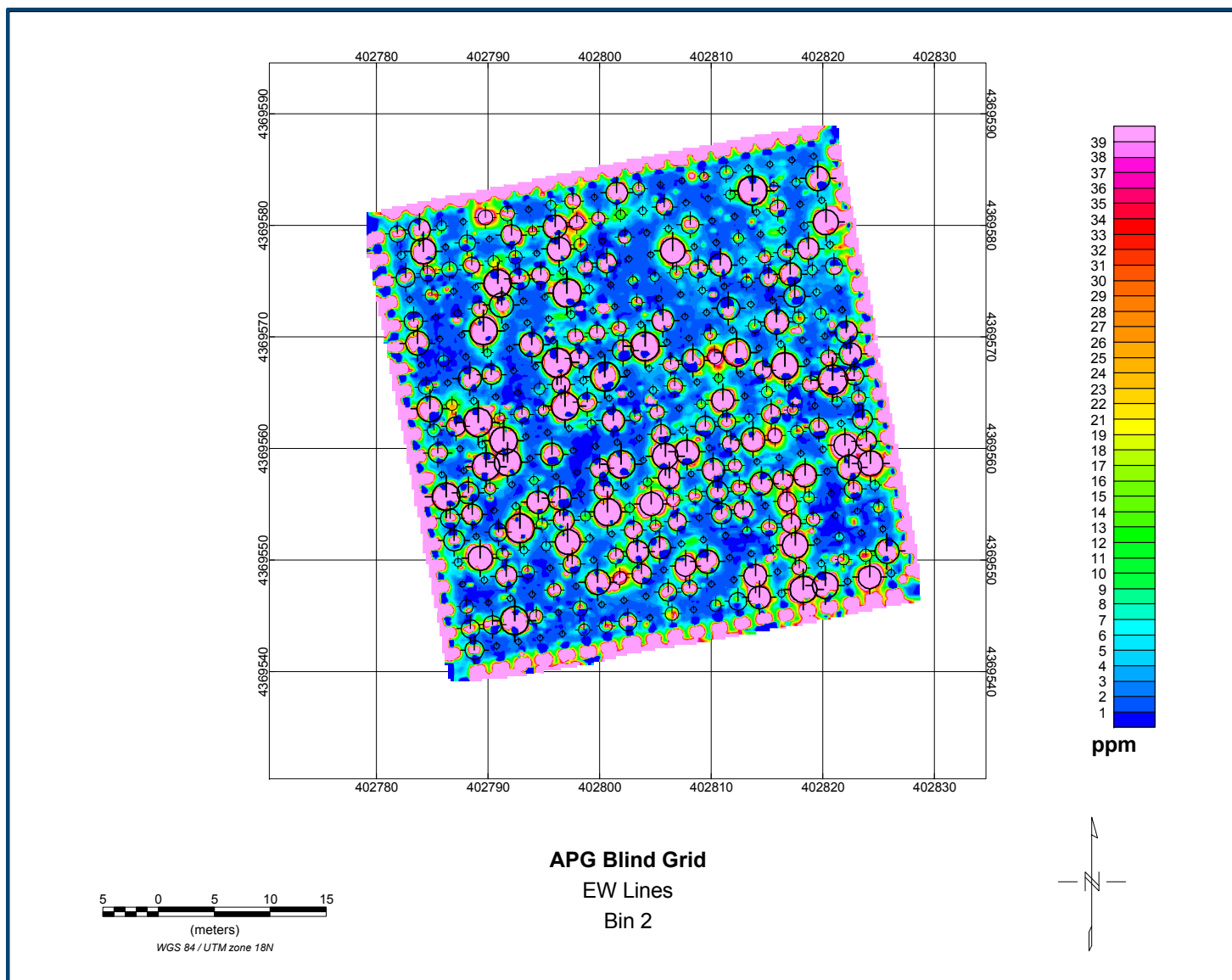
Figure 19: Plot of Bin2 response at APG Calibration Grid.
