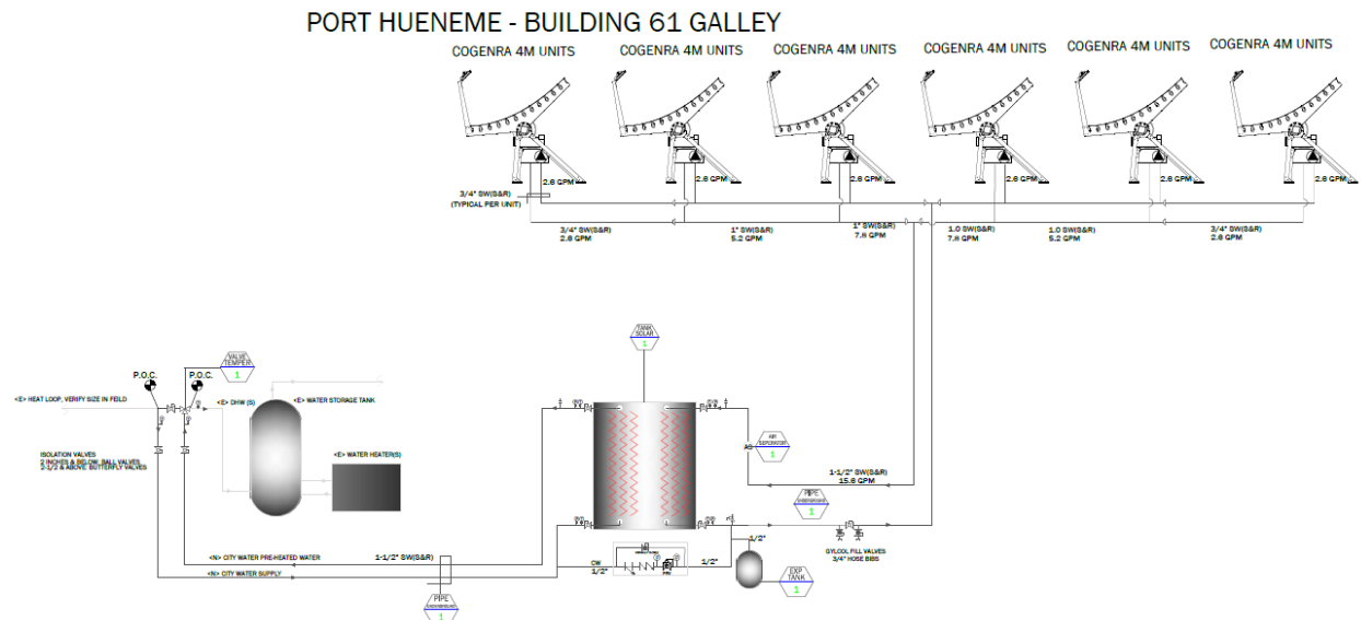
Figure 17: System hydronics configuration, including the solar tank and the existing hot water tank and heater.
