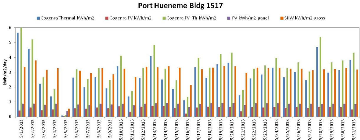
Figure 24: Cogenra system PV and thermal energy output per square meter per day, along with reference PV and SHW systems, for Port Hueneme Barracks 1517.
