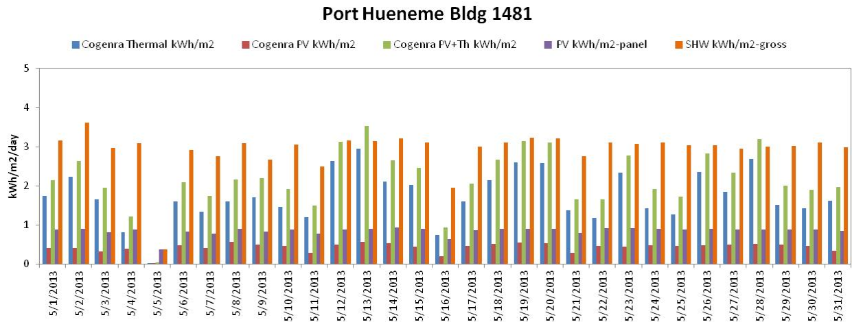
Figure 23: Cogenra system PV and thermal energy output per square meter per day, along with reference PV and SHW systems, for Port Hueneme Barracks 1481.
