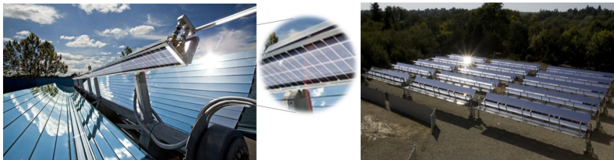
Figure 1: (left) Cogenra's original SunBase solar array configured from ground-mounted applications. (right) Commercial system (272 kWp) operating at the Sonoma Wine Company in Graton, CA.
