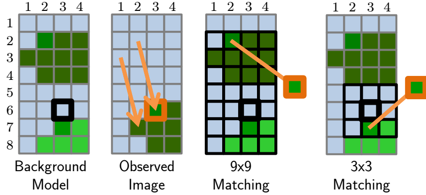
Figure 2-7: Exploiting Repetitive Texture : Consider a background model with one Gaussian per pixel learned from a stationary pair of leaves against the blue sky (leftmost image). We will be concentrating on what happens at the pixel location with the bold outline. Suppose a sudden gust of wind moves the top leaf down and right, as shown in the middle-left image. We now wish to find the best matching background Gaussian for the pixel outlined in brown. To match the Gaussian that actually generated it, we would need to have a 9 \times 9 window (middle-right image); however, a smaller 3 \times 3 window allows matching to a similar leaf in the model and labeling the pixel as background. When the dynamic textures are spatially repetitive, windows too small to capture all their movement can still be useful.
