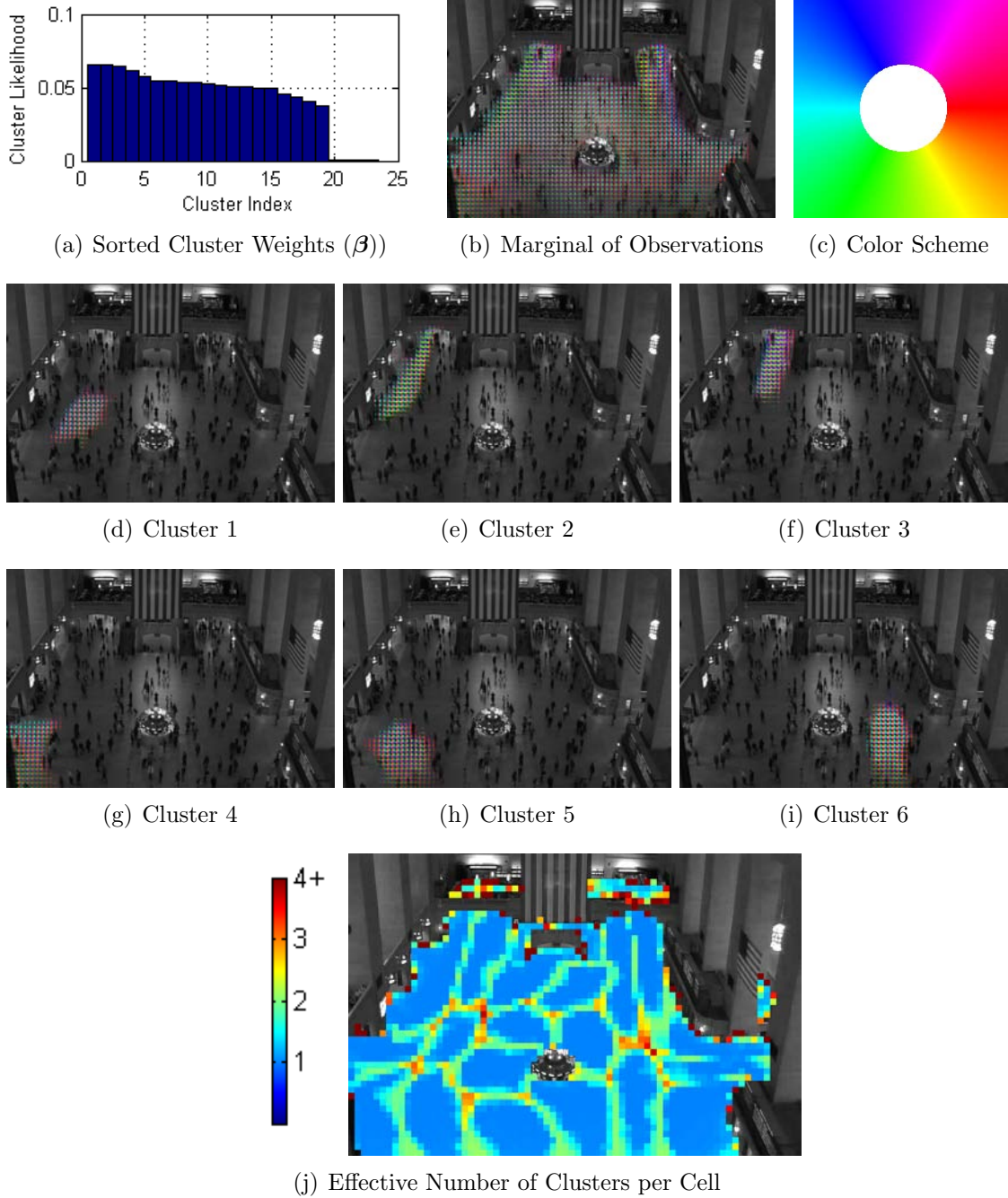
Figure 4-2: Activity Modeling with Feature Points : In Fig. 4-2(a), we show the learned activity cluster mixing weights, after sorting them. In Fig. 4-2(b), we show the marginal distribution of all observations (quantized location and moving direction of a tracked feature point) in the dataset. The hue mask in Fig. 4-2(c) encodes direction, and its alpha matting with respect to the background image encodes the observation frequency. Fig. 4-2(d)–4-2(i) show the six most highly weighted clusters. Note that although each cluster does have good spatial compactness, it captures motion in all directions. The model is unable to learn overlapping clusters where people are traveling on different paths. Except for a few of the low-weighted ones (which are not shown here), the remaining 17 clusters are qualitatively similar. In Fig. 4-2(j), we see that there is only a single cluster representing motion at most locations on the concourse floor.
