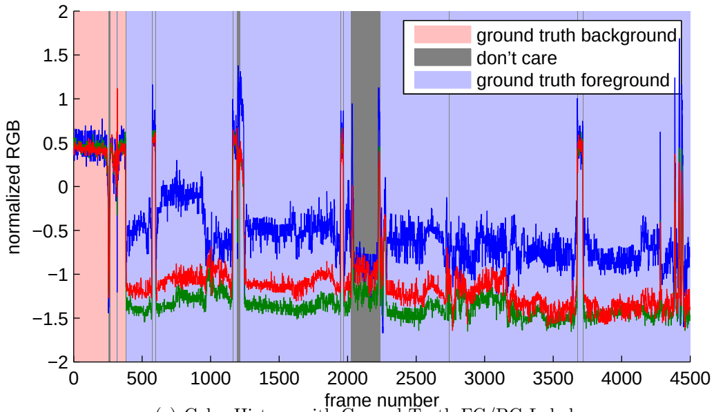
(c) Color History with Ground Truth FG/BG Labels
