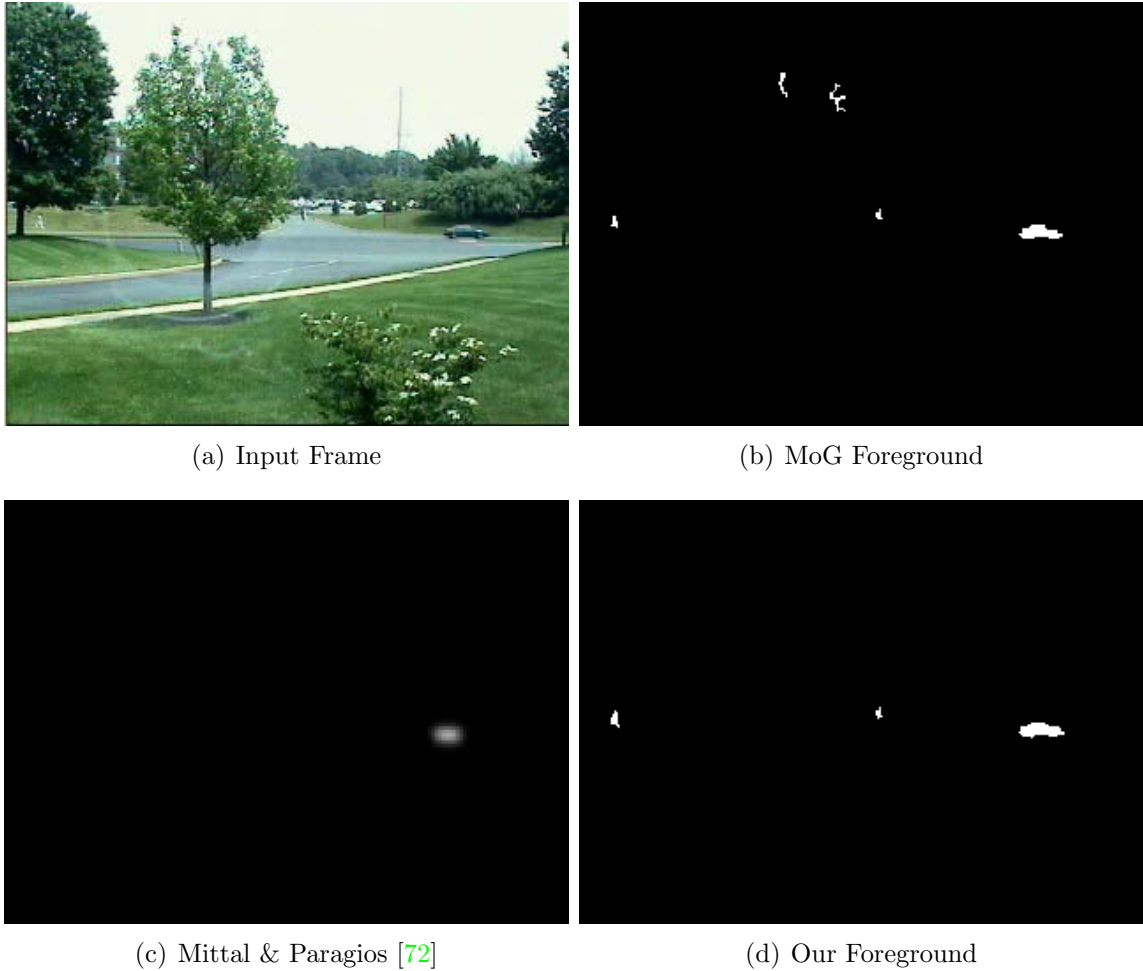
Figure 2-1: Foreground Classification Comparison: Our method is able to suppress the two false positive waving tree foreground blobs seen in the MoG results. We are simultaneously able to retain the two very small pedestrians, unlike the previously best results on the video.
