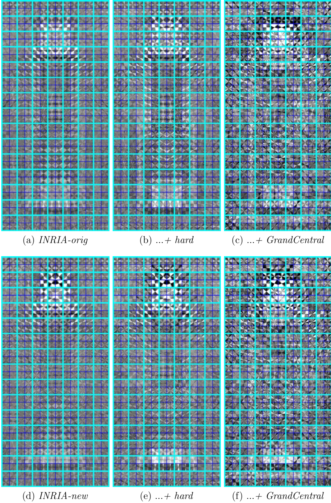
Figure 3-18: Classifier Renderings : Here we show renderings of the \mathbf{w} portion (see Eqn. 3.8) of several learned classifiers (see Tab. 3.4).
