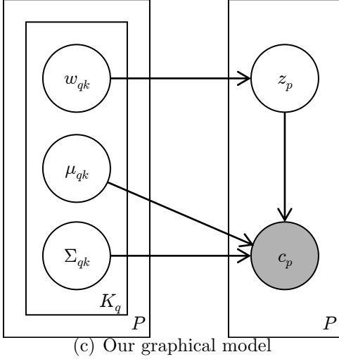
Figure 2-2: Traditional MoG Model vs. Ours : In Fig. 2-2(a) and Fig. 2-2(c), we show a graphical model representation of the traditional Mixture of Gaussians (MoG) background subtraction model and our model, respectively. Circles represent random variables, shaded circles represent observed values, and plates indicate replication of random variables which are independent except where there are arrows. In the traditional MoG model, the color c_q observed at pixel q is generated from a randomly-selected mixture component at the same pixel location. A given mixture component can at most influence the observed color for a single pixel (see Fig. 2-2(b)). In our model, c_q is sampled from mixture components at location q as well as components located at neighboring pixels. Each mixture component can influence the observed colors within some local neighborhood (a 3 \times 3 neighborhood is shown in Fig. 2-2(d)). This extra spatial neighborhood allows our model to more gracefully handle backgrounds that undergo small local motions. See the text for precise definitions of the random variables.
