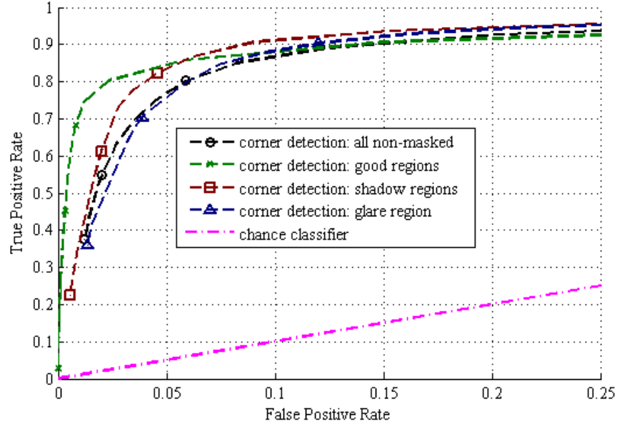
(a) Regional Corner Detection ROC Curves
