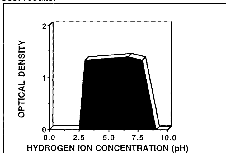
Figure 21. The pH range over which all copper is converted to copper (I) in this study.
