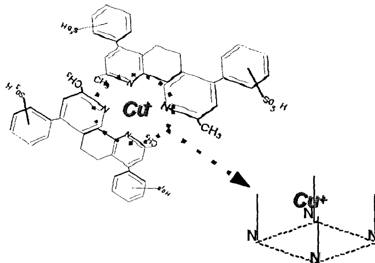
Figure 10. Copper (I) complexed between the nitrogens of BCS molecules that are at right angles to each other.
