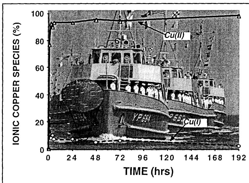
Figure 23. Leaching profile of Woolsey Neptune Red.
