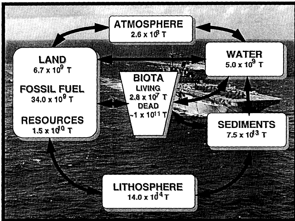
Figure 7. Global copper cycle (redrawn from Nriagu 1979).
