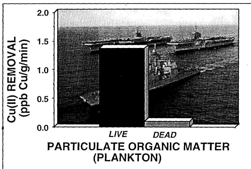
Figure 25. Organic ligands added to samples containing ionic copper.
