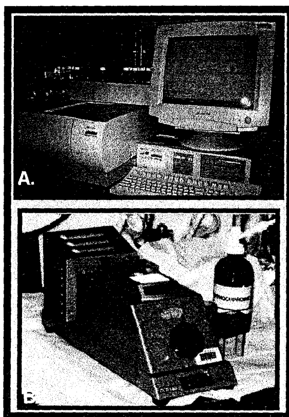
Figure 9. Set-up for measuring the results of the copper (I) reaction. A=spectrophotometer; B=colorimeter.
