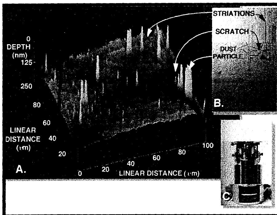
Figure 33. The results of using an Atomic Force and a Light microscopy to determine how the ionomeric Nafion 117 membrane probe responds to treatment. A=Atomic Force analysis of membrane surface with BCP imbedded and treated with Cu(I); B=Light microscope view of membrane surface before cleaning and chemical treatment; C=Atomic Force Microscope (AFM).
