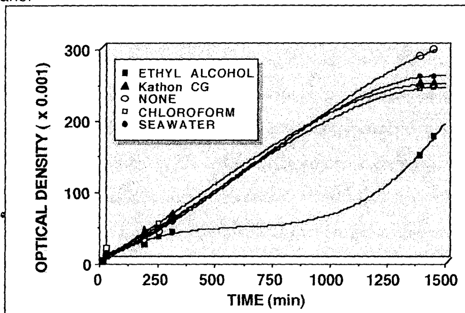
Figure 40. The effect of preservative on the membrane and its ability to uptake Cu(I).
