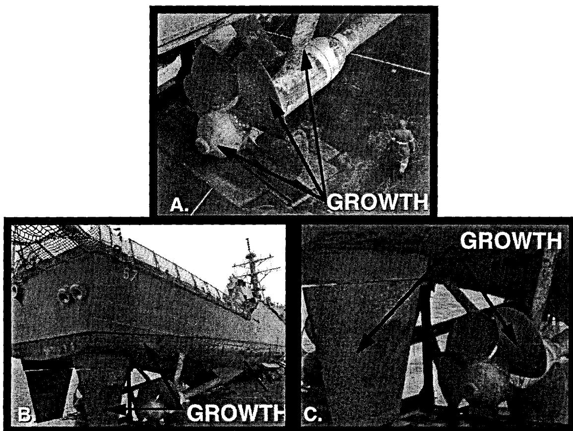
Figure 2. Shipboard bio-fouling occurring even in areas of strong currents.
