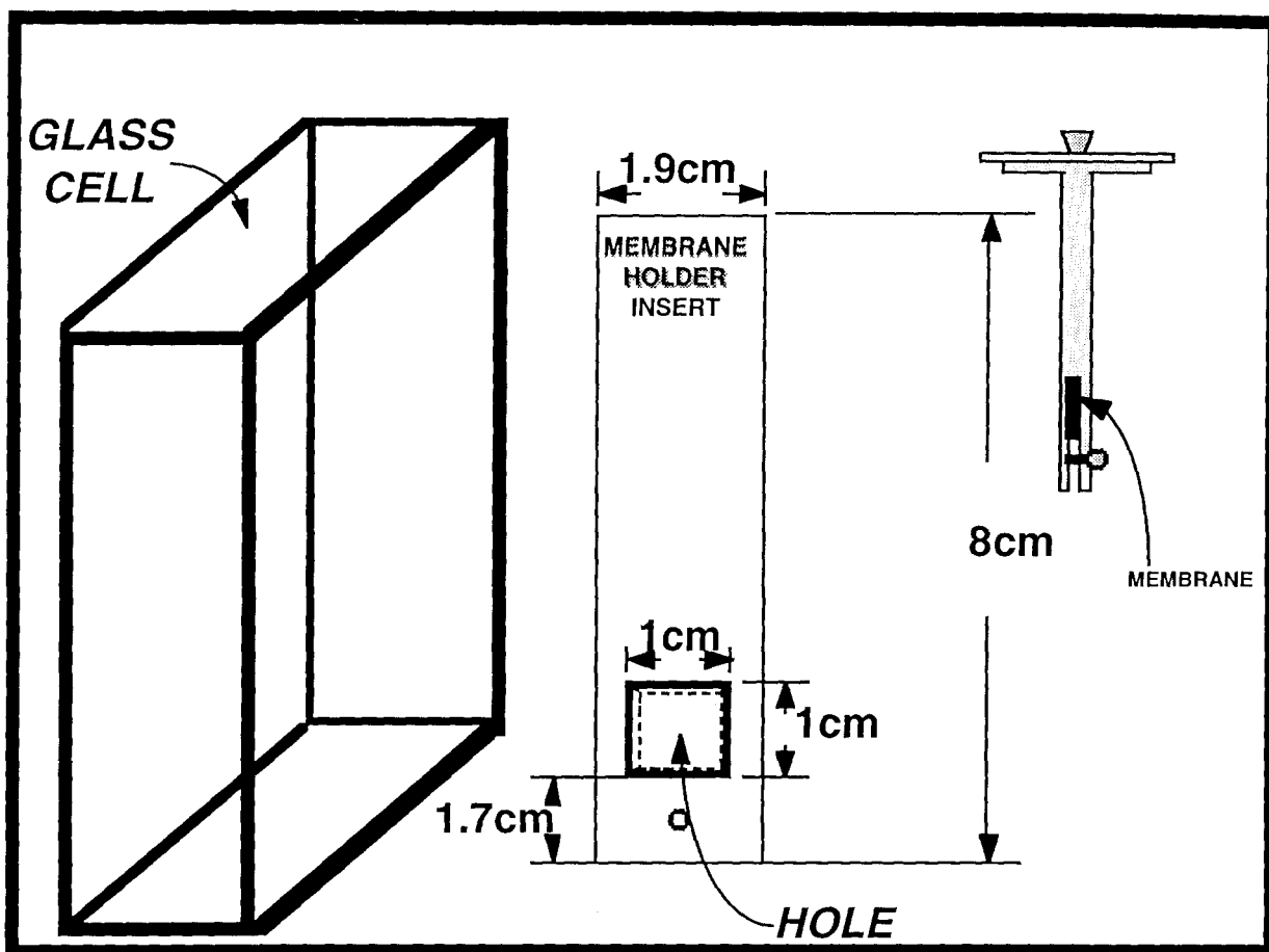
Figure 15. Specially constructed Teflon membrane holder used to test Cu(I) uptake into Nafion membrane.
