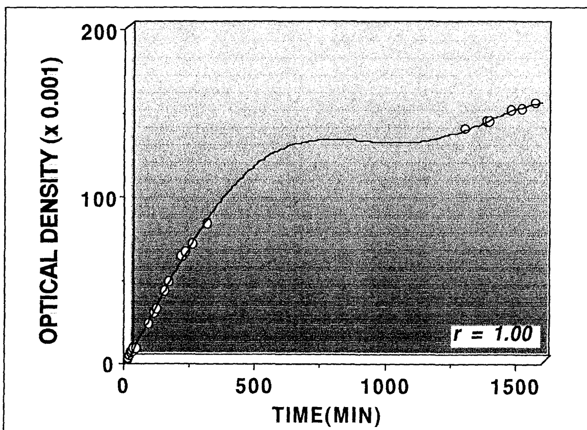
Figure 29. Response of ionomeric Nafion 117 membrane probe imbedded with BCP to the presence of 1000ppb of Cu(I).
