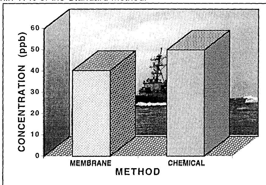
Figure 19. Comparison of the result from testing the Nafion 117 membrane impregnated with BCP to the Bathocuproine Method (Clesceri et al 1998).
