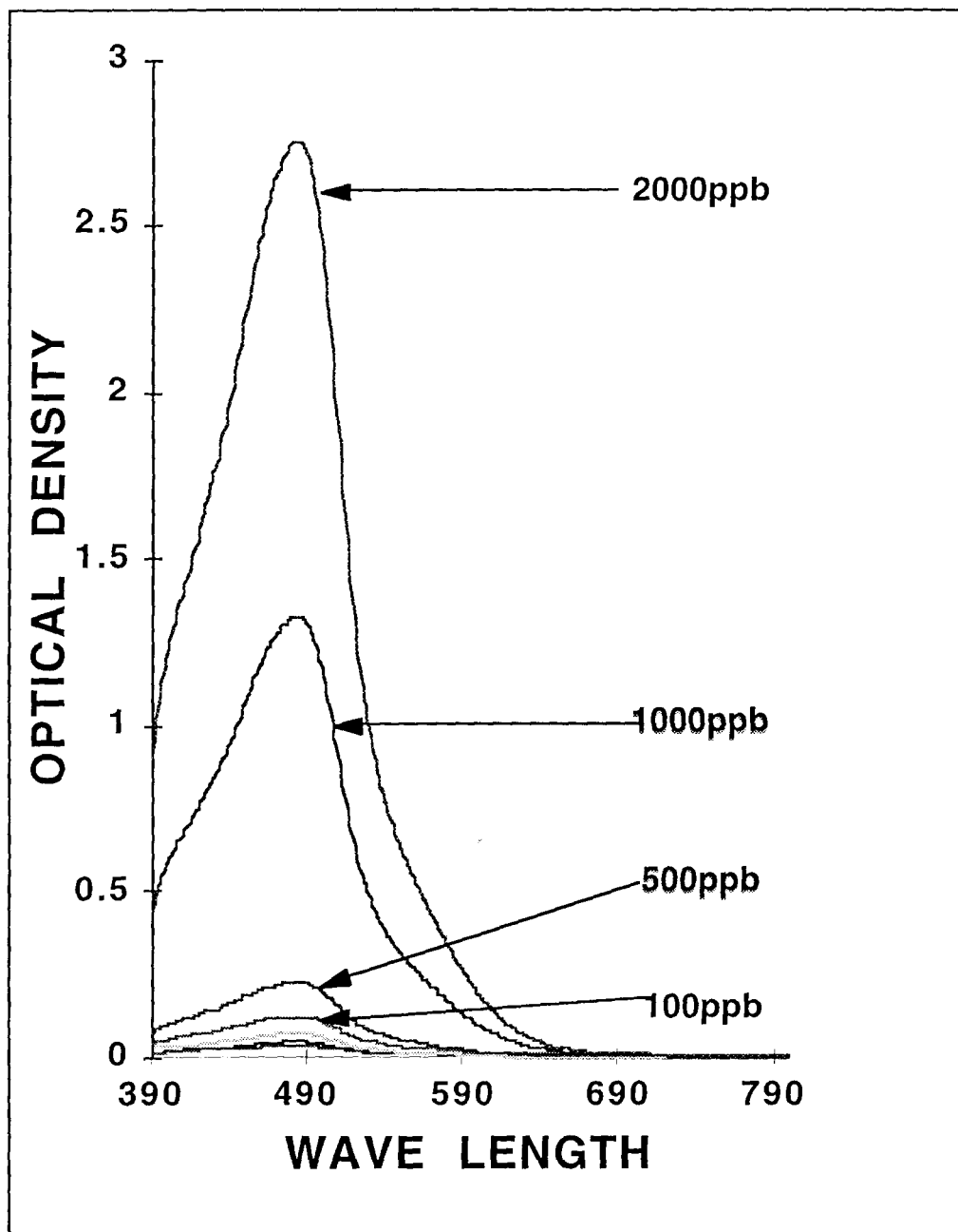
Figure 22. Scanning spectrophotometer plots of Copper (I) concentrations from 10 to 2000ppb.
