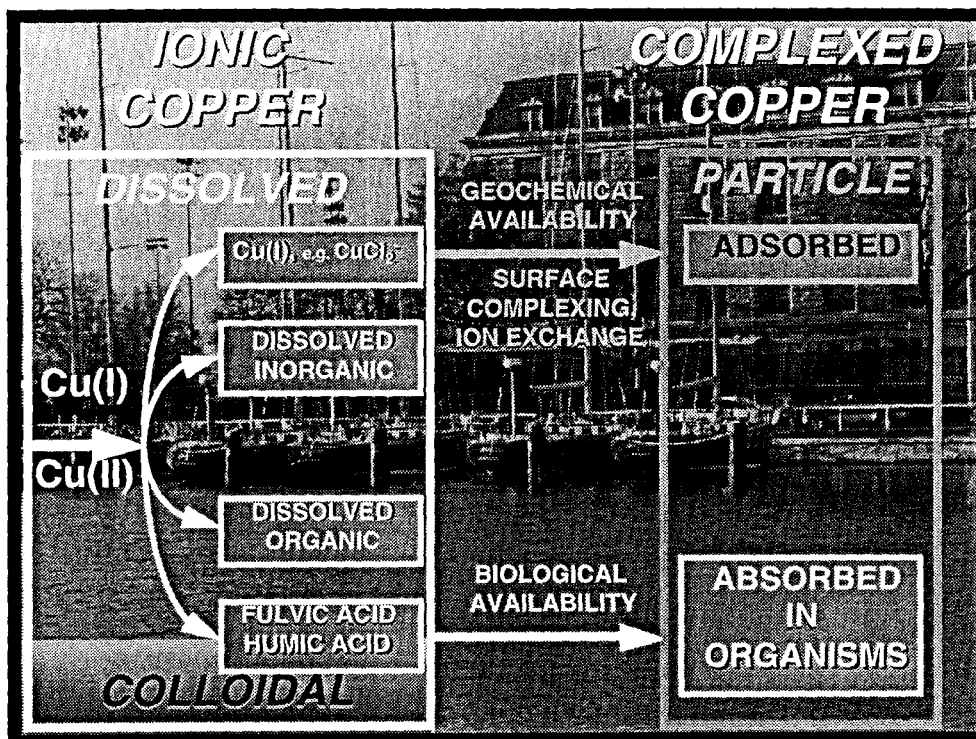
Figure 17. Reaction pathways for ionic copper in the aquatic environment.
