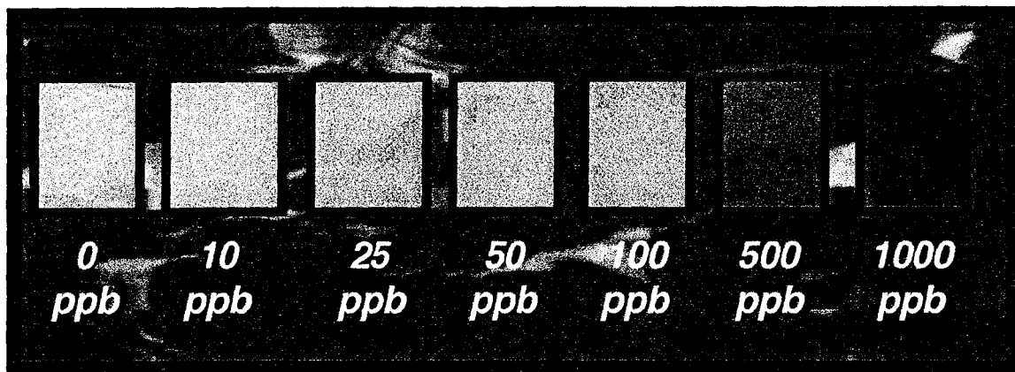
Figure 32. Comparison of orange intensity from actual membranes placed in varying concentrations of Cu(I) for 24 hours at 25°C in de-ionized water on an orbital shaker revolving at 100 revolutions/ minute.
