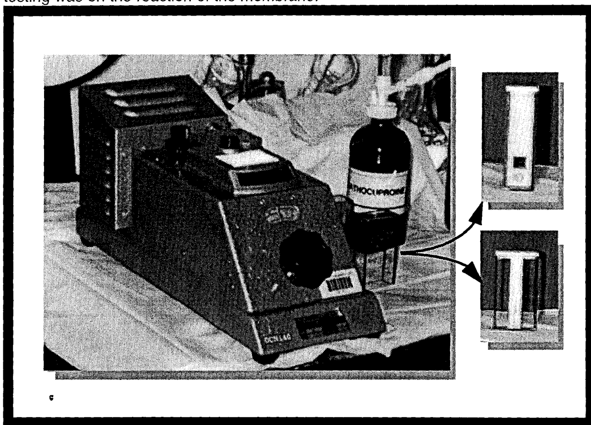
Figure 14. Colorimeter with 4.4cm cell and teflon membrane holder.
