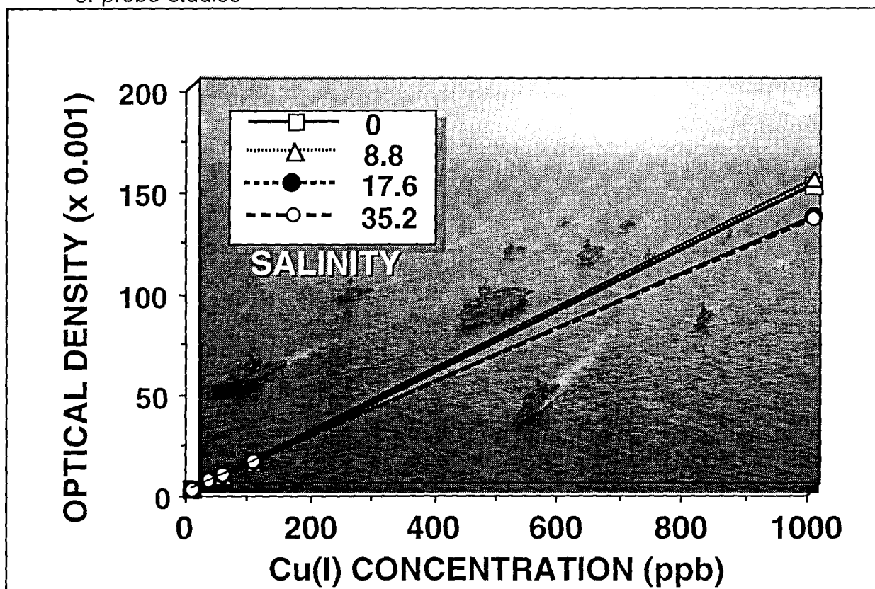
Figure 11. Calibration curves for various salinity waters.
