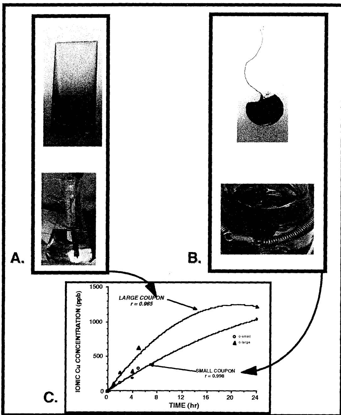
Figure 12. Ionic copper source from Navy used Interviron anti-fouling coating and Woolsey Neptune Red. A=Glass coupon with Interviron; B=Glass coupon with Woolsey Neptune Red; C=Leaching response of glass coupons with copper containing anti-fouling coating.
