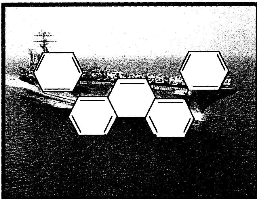
Figure 8. Bathocuproine=BCP(2,9-dimethyl-4,7-diphenyl-1,10-phenanthroline) (redrawn from Diehl and Smith1972).
