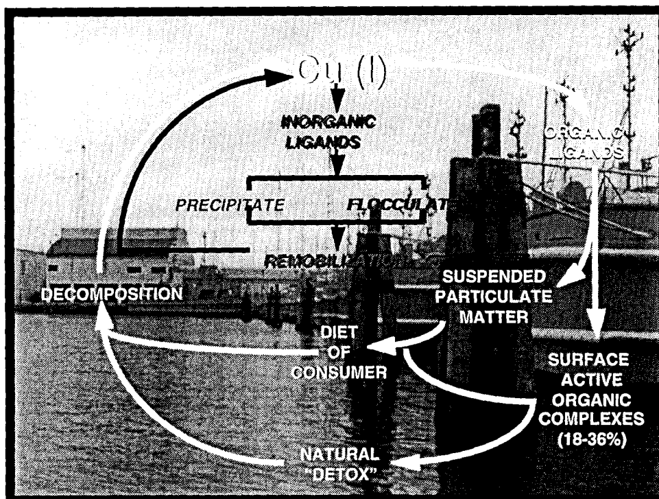
Figure 18. Cu(I) circulation through the aquatic habitat.
