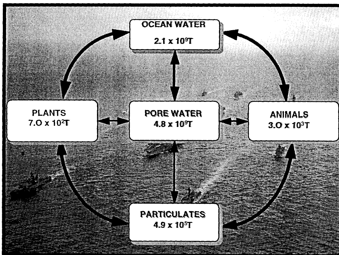
Figure 6. Ocean copper cycle (data from Nriagu 1979).
