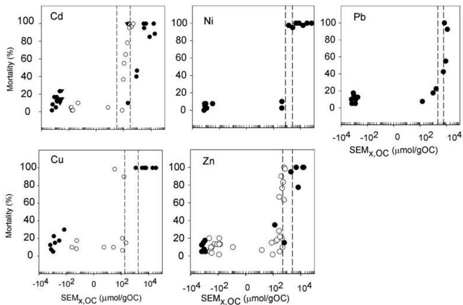
Figure 14. Comparison of Predicted and Observed Amphipod Mortality. The Dashed Lines are the Predicted D. magna LC50s for pH = 6 and pH = 9. The Data are Amphipod Mortality Versus Organic Carbon Normalized Excess SEM_{X,OC} = (SEM - AVS) / f_{OC} (Eq. 4) (Di Toro et al., 2005b)
