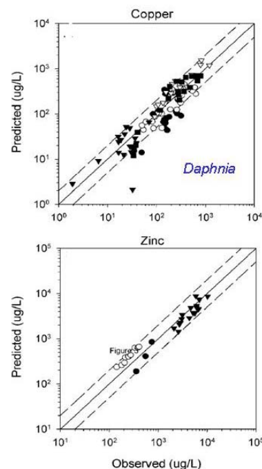
Figure 4. Schematic of the Biotic Ligand Model (left) (Di Toro et al., 2001; Santore et al., 2001). Application of the BLM to D. magna for Cu and Zn (right) (Di Toro et al., 2005b).
